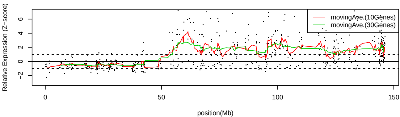
LC_C13 Chr8
