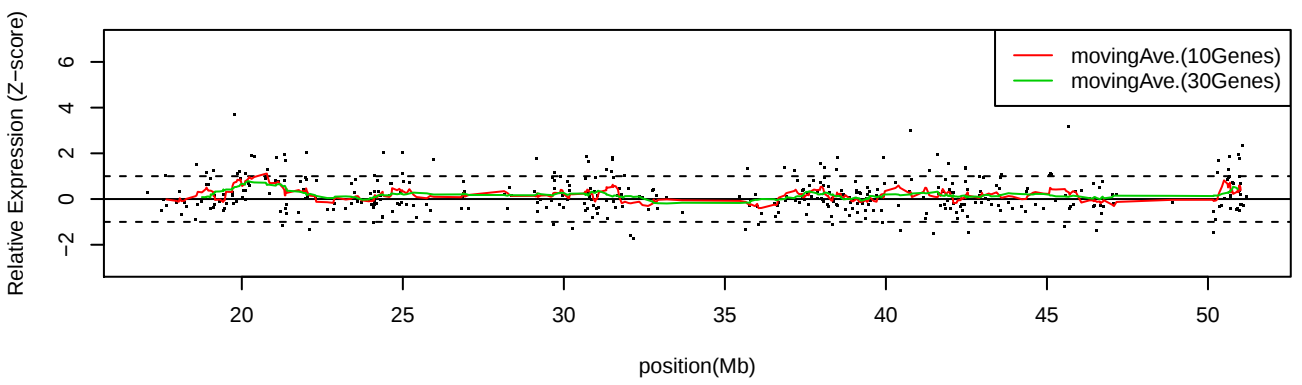
LC_C14 Chr22
