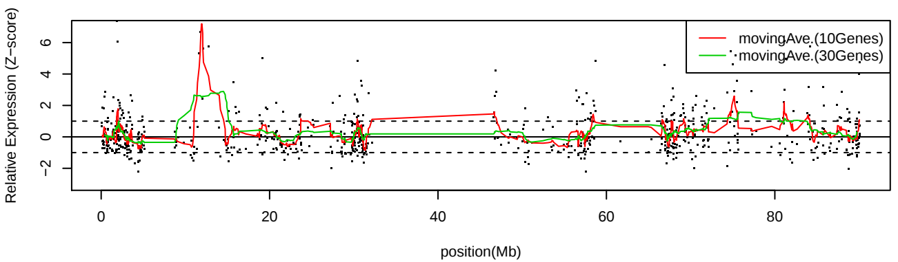
LC_C18 Chr16
