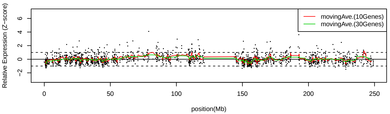
LC_C12 Chr1
