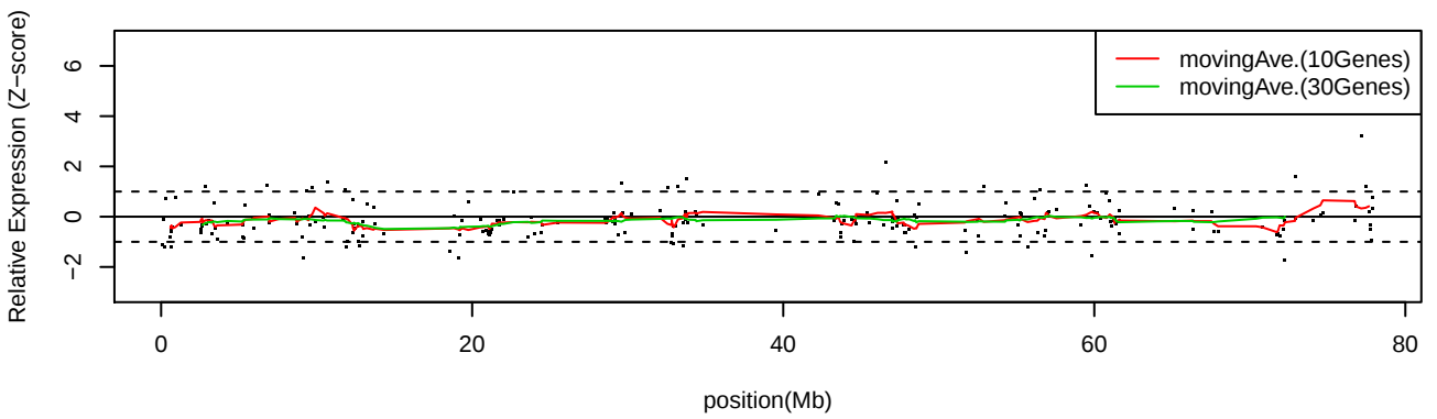
LC_C20 Chr18
