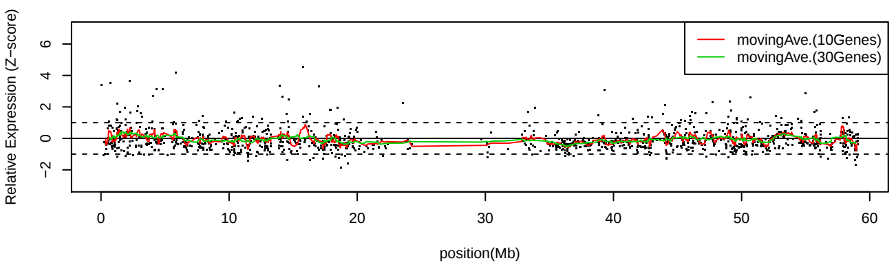
LC_C19 Chr19
