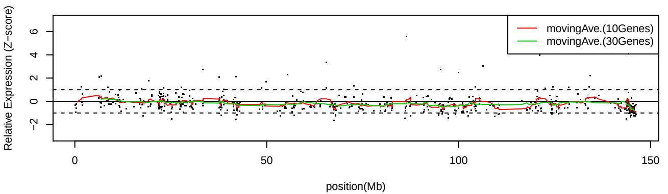
LC_C20 Chr8
