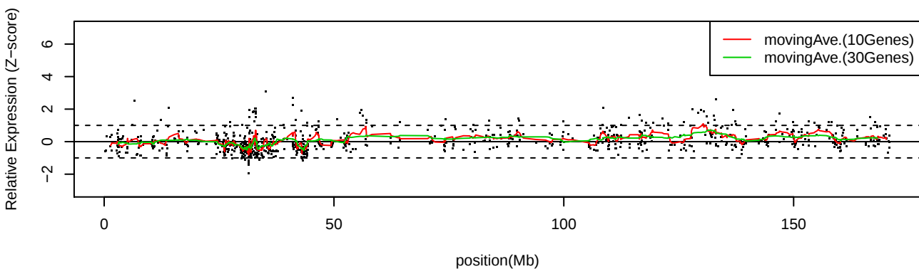
LC_C12 Chr6
