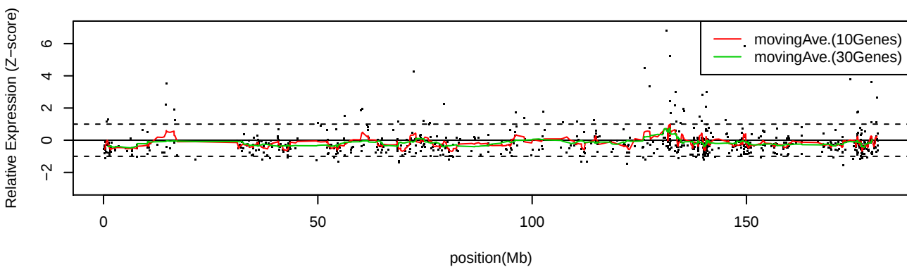
LC_C19 Chr5
