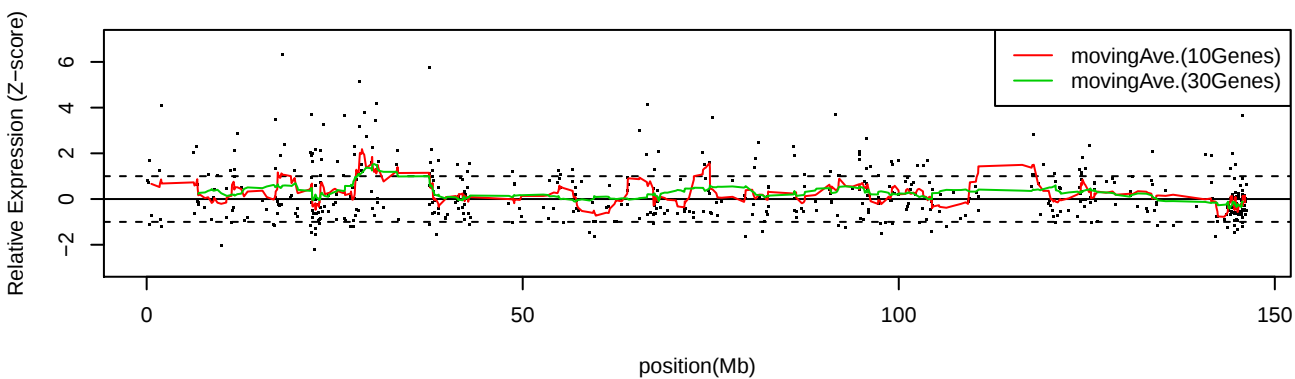
LC_C18 Chr8
