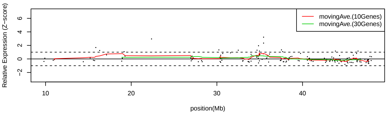
LC_C12 Chr21
