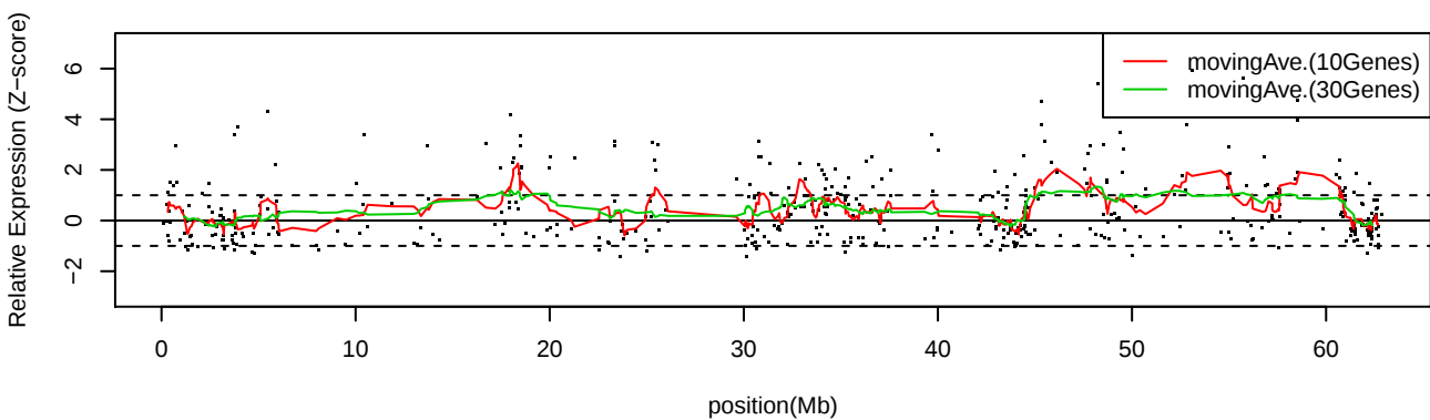
LC_C18 Chr20
