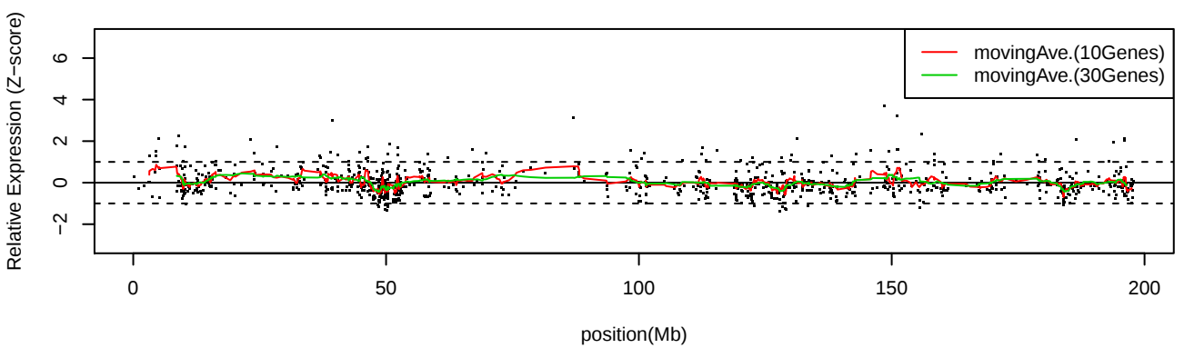
LC_C12 Chr3
