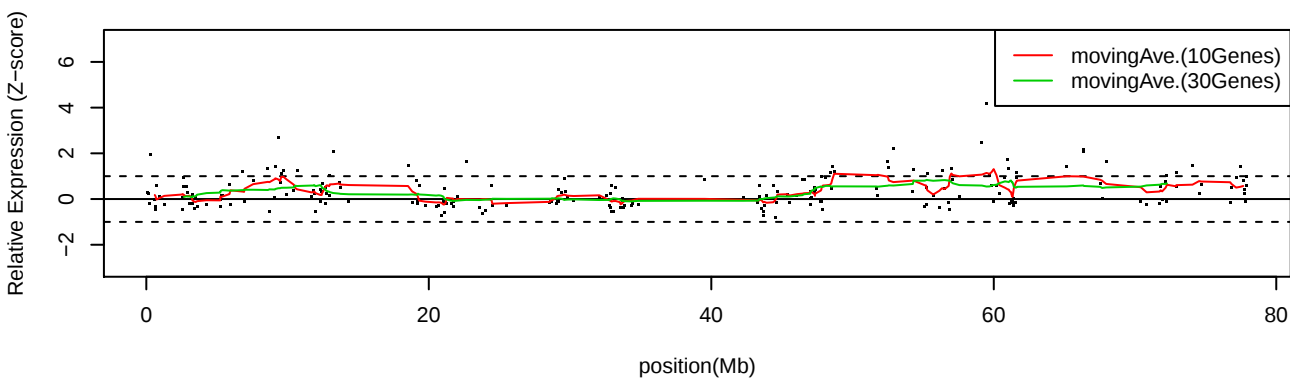
LC_C17 Chr18
