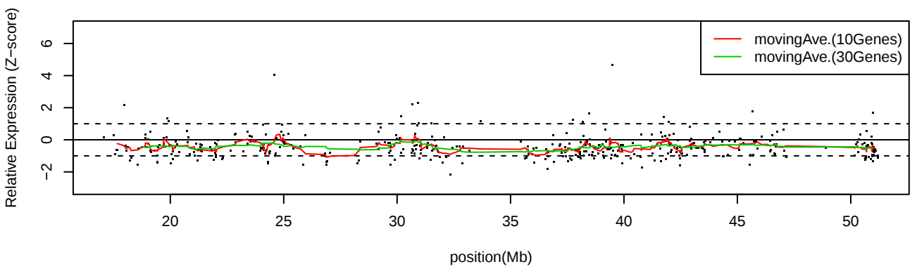
LC_C15 Chr22
