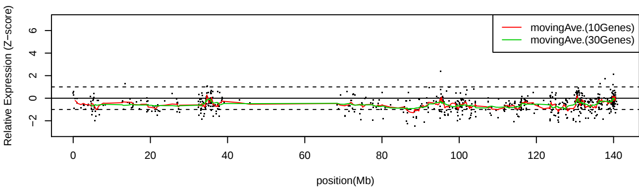
LC_C14 Chr9
