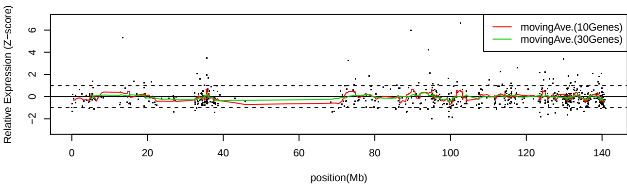
LC_C20 Chr9
