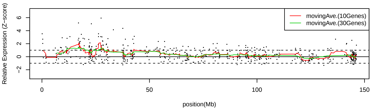
LC_C15 Chr8
