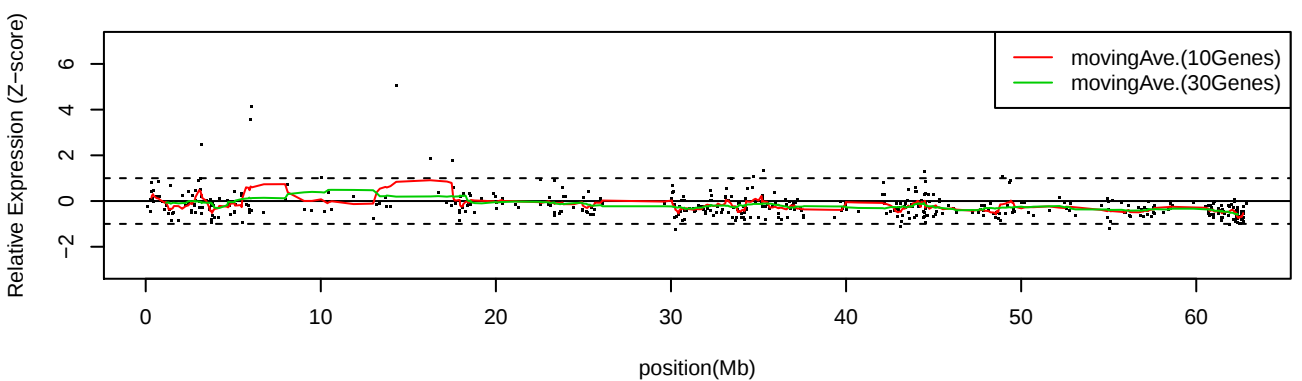
LC_C11 Chr20
