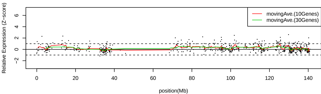
LC_C17 Chr9
