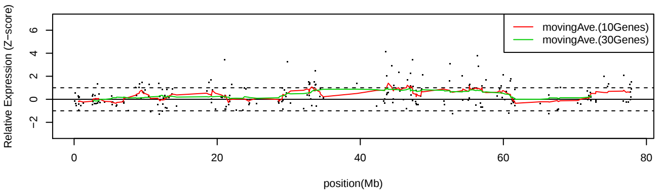
LC_C13 Chr18
