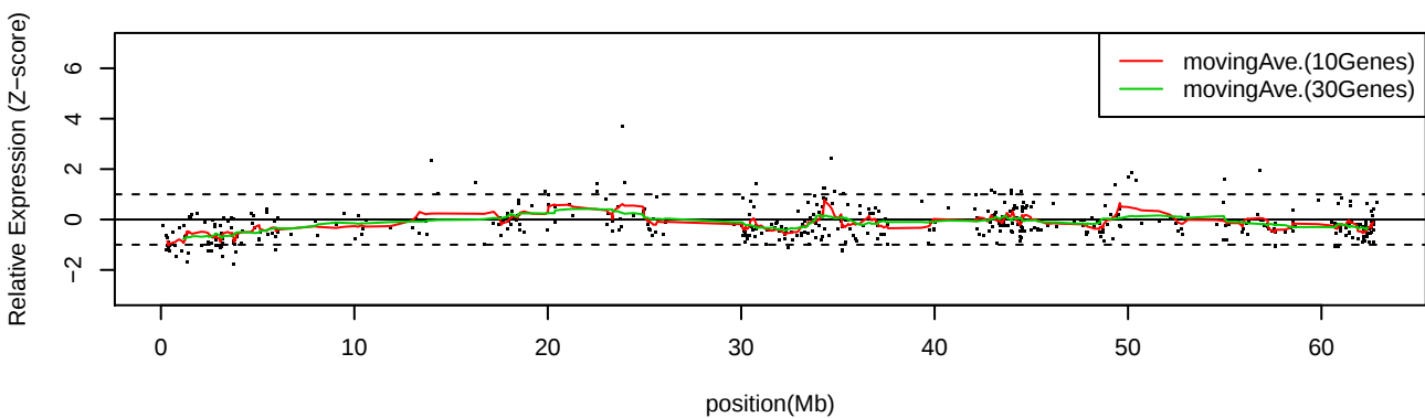
LC_C16 Chr20
