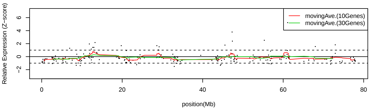
LC_C19 Chr18
