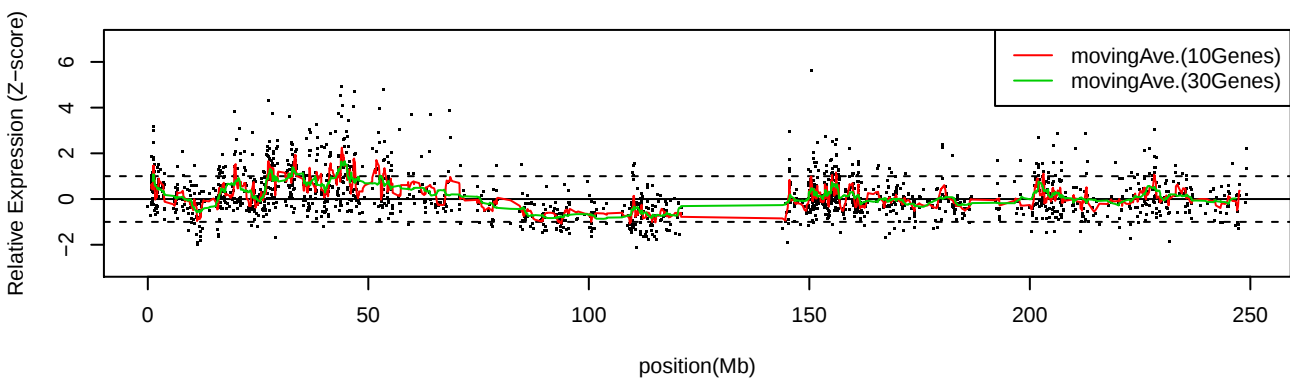
LC_C14 Chr1
