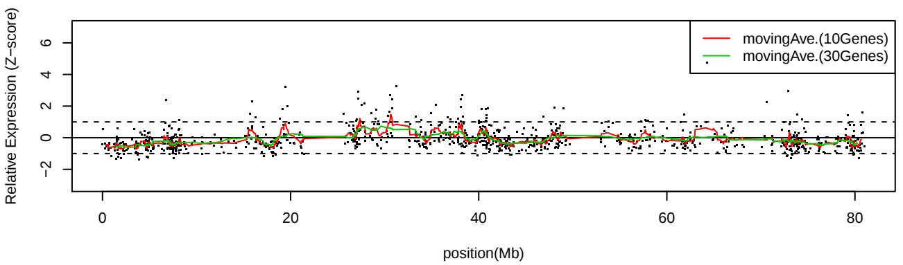
LC_C11 Chr17
