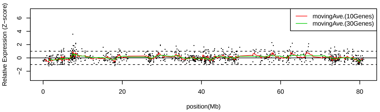
LC_C12 Chr17
