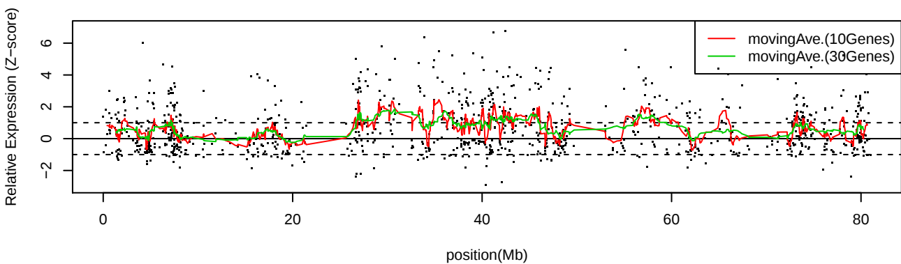
LC_C18 Chr17
