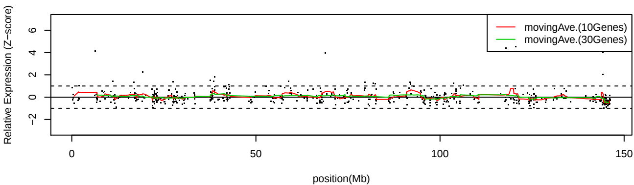
LC_C17 Chr8
