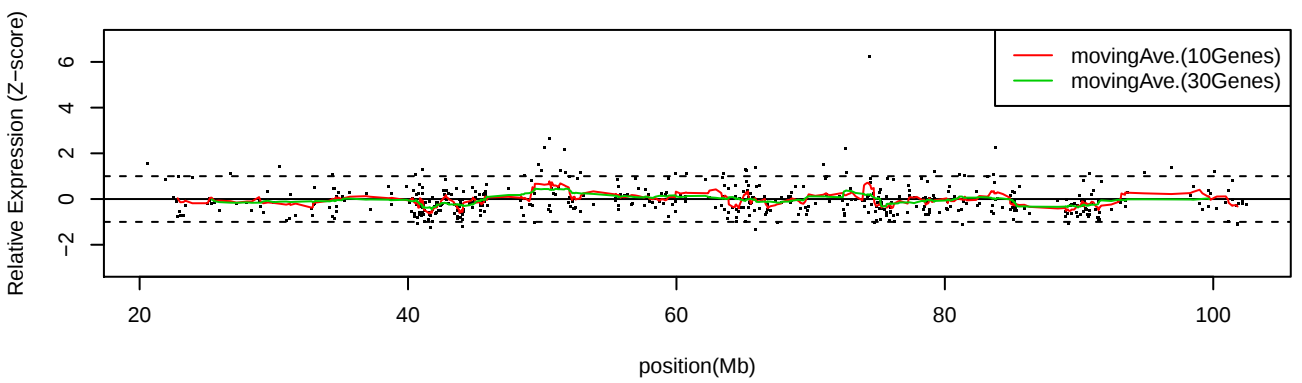
LC_C12 Chr15
