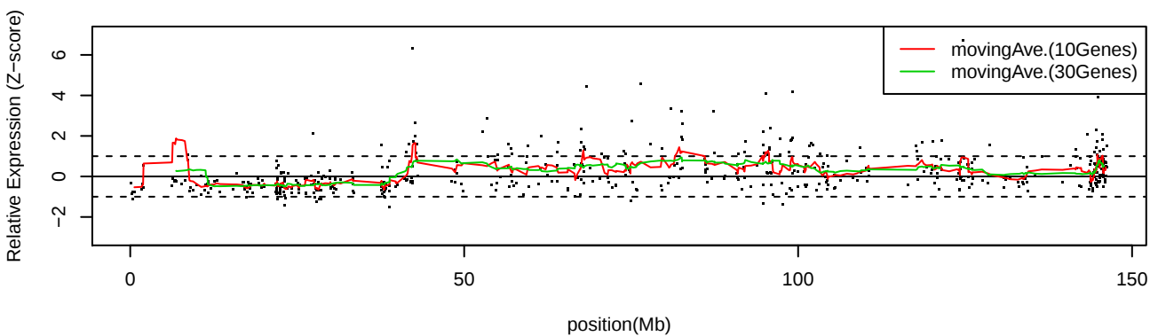
LC_C19 Chr8
