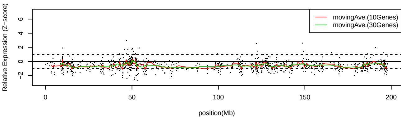
LC_C14 Chr3
