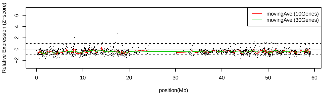
LC_C11 Chr19
