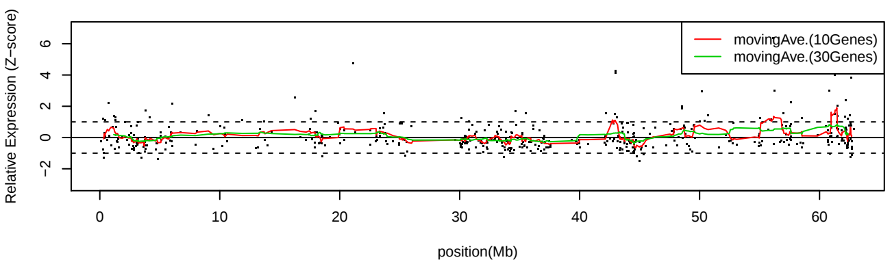
LC_C19 Chr20
