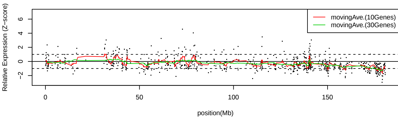
LC_C18 Chr5
