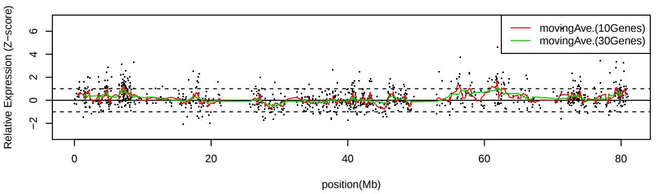
LC_C14 Chr17
