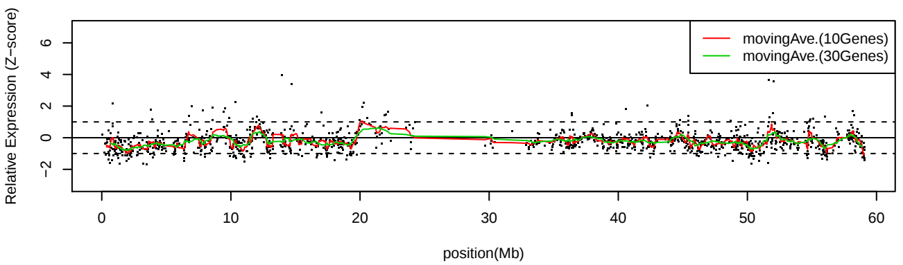
LC_C12 Chr19
