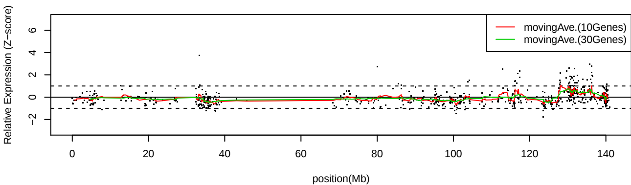
LC_C11 Chr9
