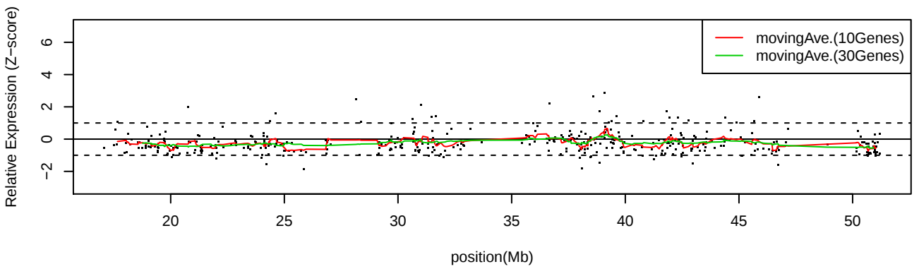
LC_C20 Chr22
