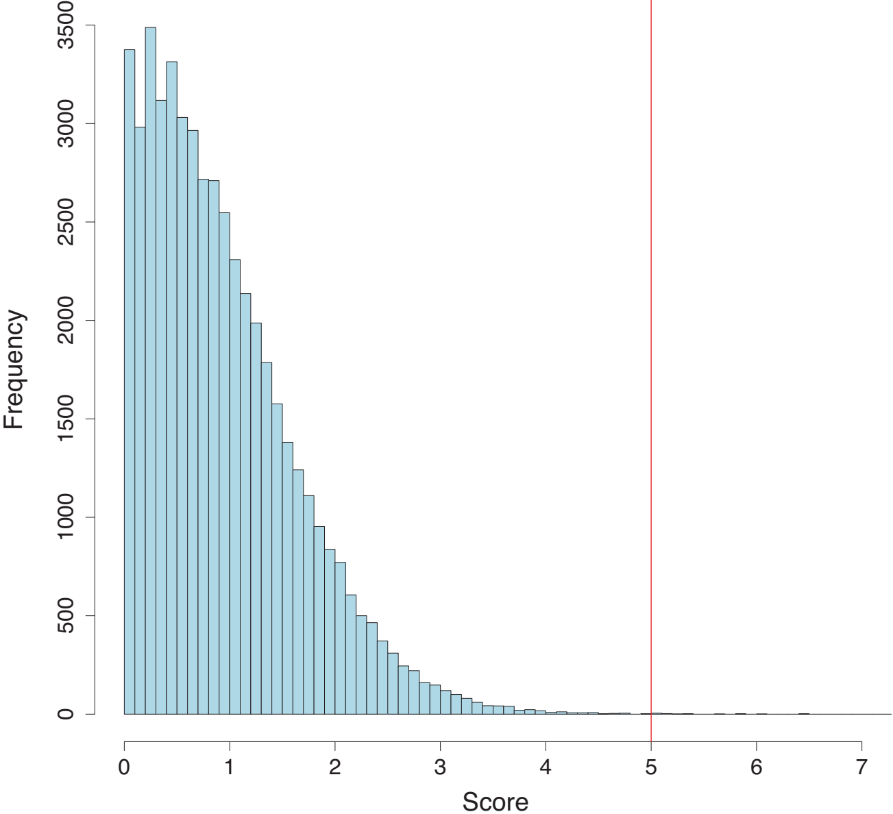
Figure S7. Distribution of scores on 50.000 random regions of the mappable mm9 mouse genome. The X axis indicate scores, the Y axis indicate the number of random regions for a given score (frequency).
