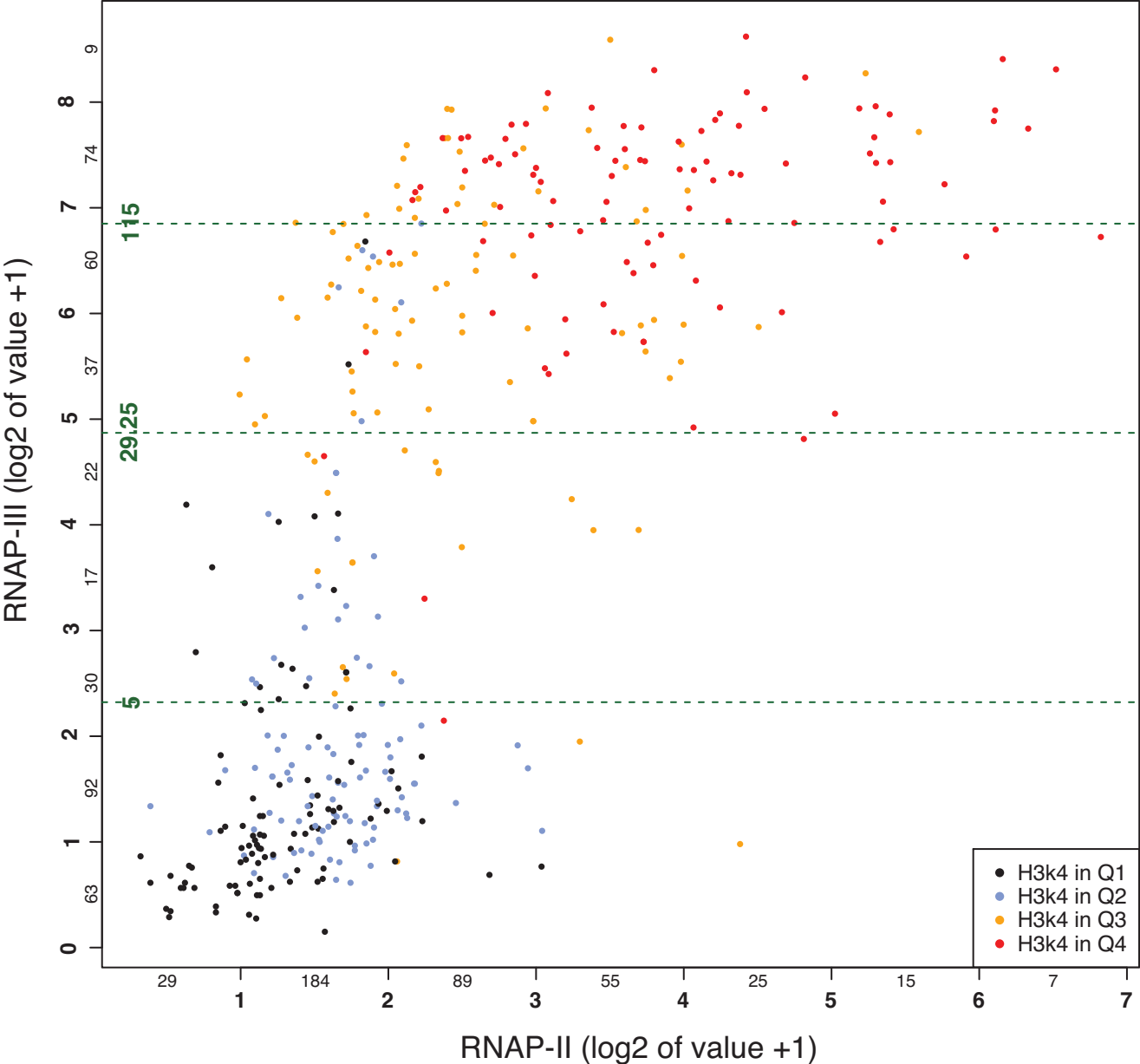
Figure S6. The X and Y axis show RNAP-II and RNAP-III scores (log2 of value+1). The numbers along the axis indicate the number of points counted in vertical respectively horizontal slices of 1 unit starting at 0. The colors of the dots indicate amounts of H3K4me3 tags at the gene, as indicate in the lower right corner.
