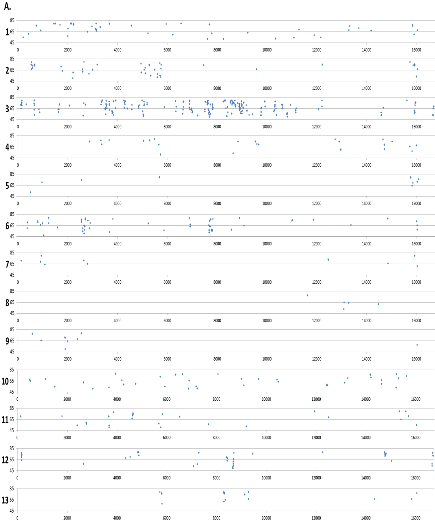
Figure S5. Biallelic SNP locations for each individual and SNP statistics. Only SNPs with minor allele frequency \geq 20\% were included. A) Major allele frequencies are plotted in their relative position across the mitochondrial genome for each individual. B) SNP Statistics.
