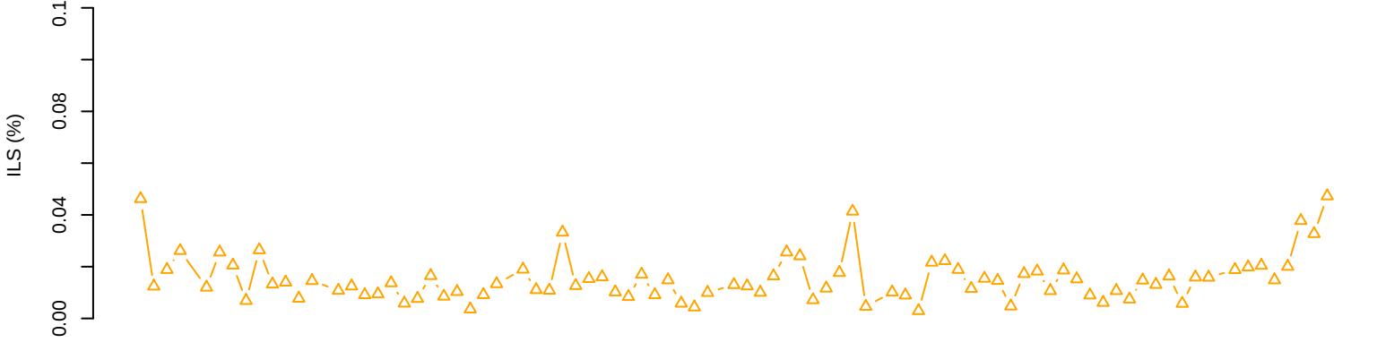
Incomplete Lineage Sorting
