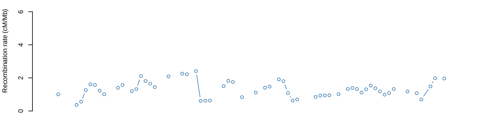
Decode Recombination Rate
