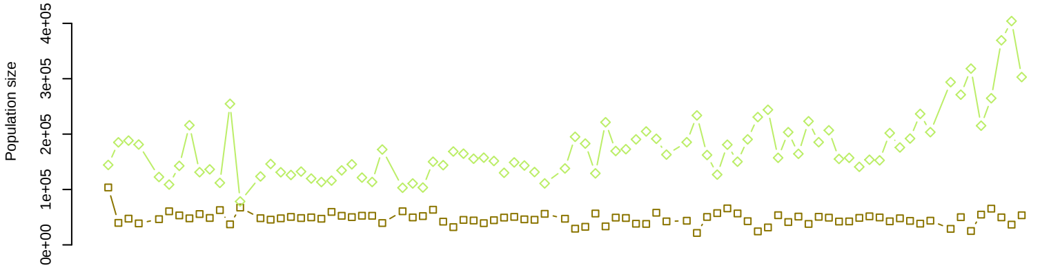
Ancestral Effective Population Size
