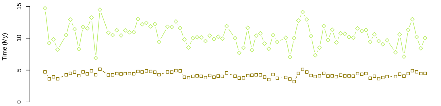
Speciation Time
