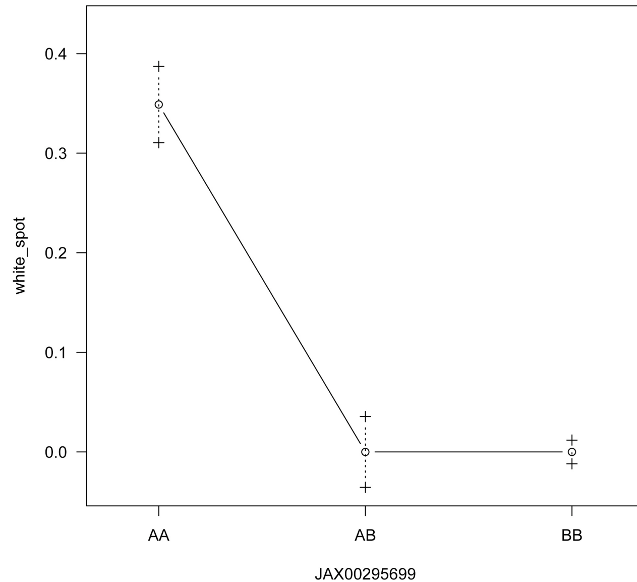
Chr 10:89.9 Mb Genotype Effects
