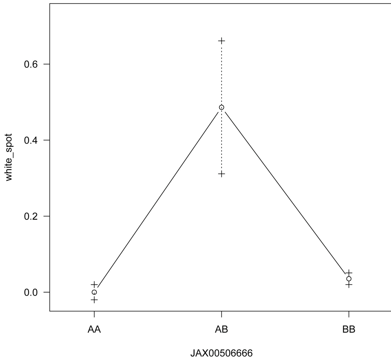
Chr 2:147.4 Mb Genotype Effects
