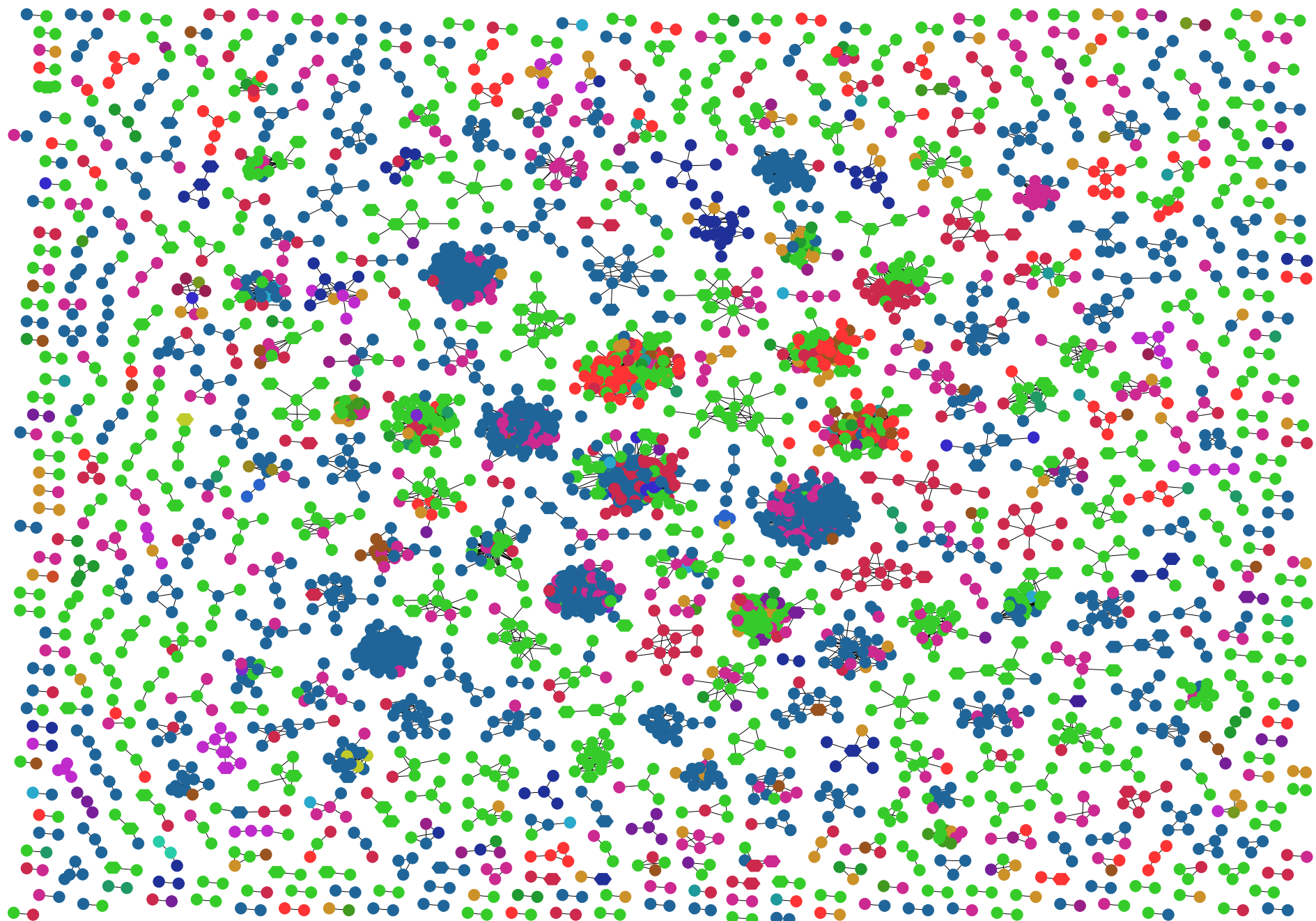
Coexisting OTUs clusters - clustd = .03 - adjusted pvalue (FDR) cut-off = 0.001
