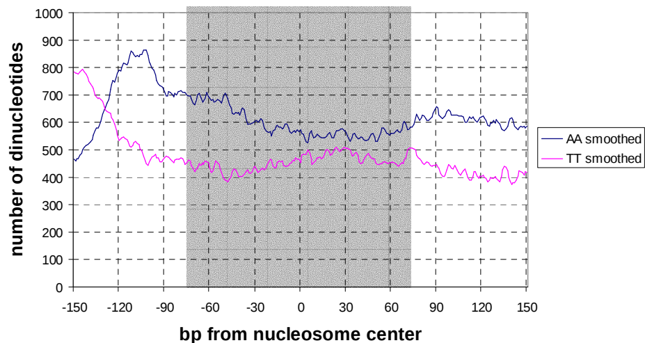
Supplementary Figure 5a – AA and TT dinucleotide counts at +1 and -1 nucleosomes flanking yeast NFRs. Shaded areas indicate nucleosome occupied (intra-nucleosomal) regions. Data is smoothed over a 3-bp window.
