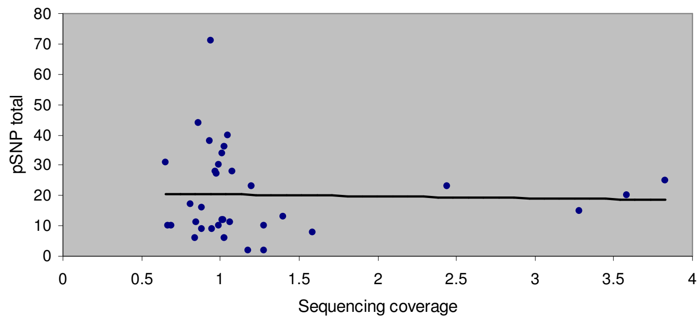
rDNA pSNP total vs coverage
