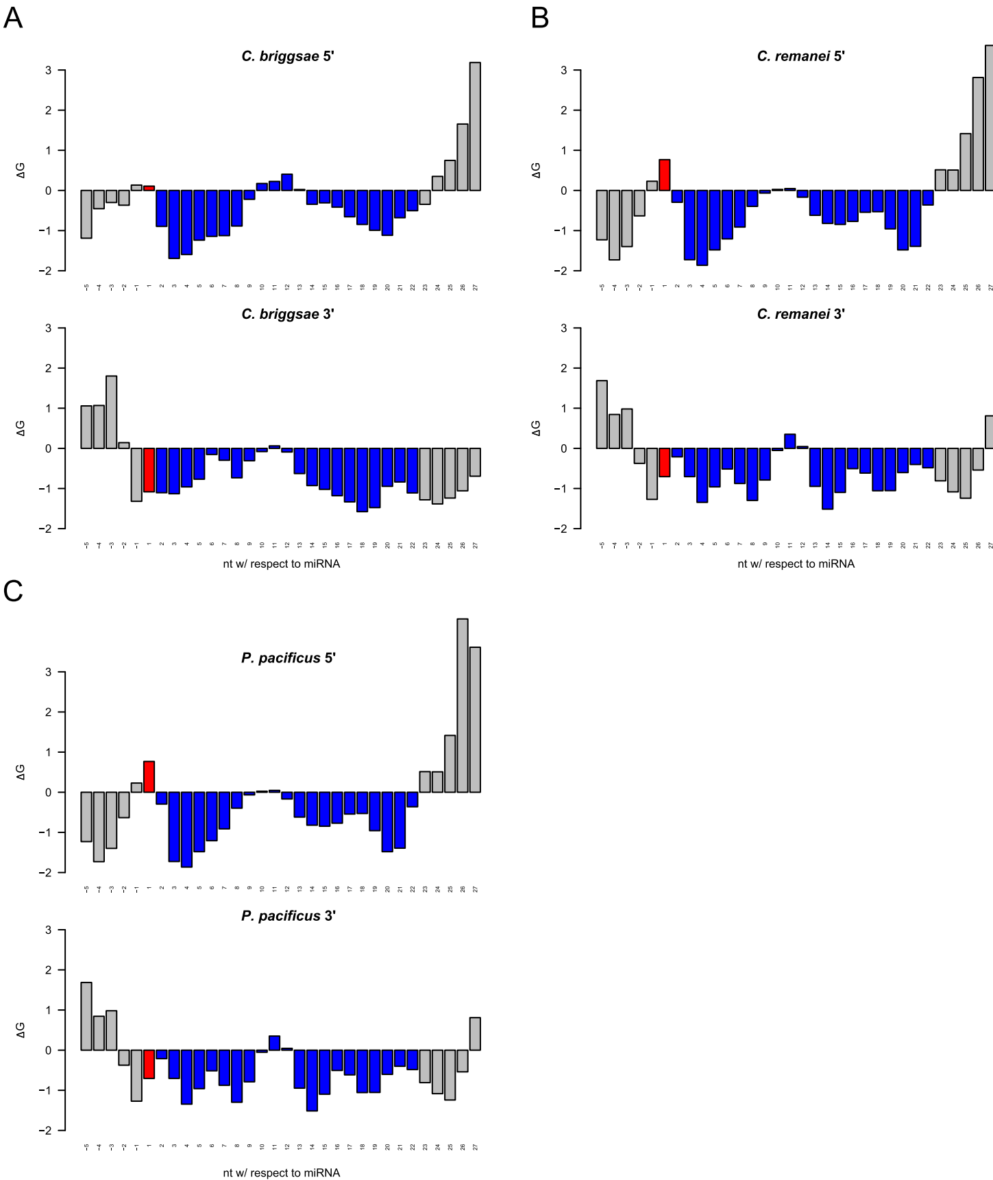
Figure S5: Thermodynamic profiles for mature miRNAs. As Fig. 2B, for C. briggsae (A); C. remanei (B); and P. pacificus (C). Positive \Delta G values denote instability in the miRNA hairpin. The red bar identifies the starting nucleotide of the miRNA, the blue bars the rest of the canonical 22 nucleotide miRNA.
