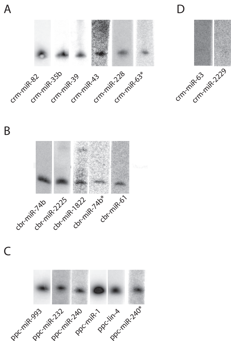
Figure S1: Northern analysis of known and candidate miRNAs. The presence of a number of randomly chosen candidate miRNAs was confirmed by Northern blotting. Out of this set of 19, of which one was known miRNAs in C. briggsae (cbr-miR-61), 17 (89%) showed a distinct band around the expected size (ca 22nt). A) C. remanei , B) C. briggsae , C) P. pacificus . Negative blots are shown in D. Probe sequences are described in the supplemental files.
