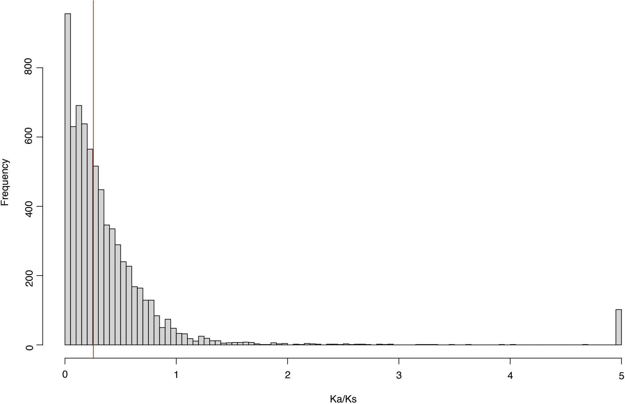
Histogram of pairwise Ka/Ks between C. immitis and C. posadasii
