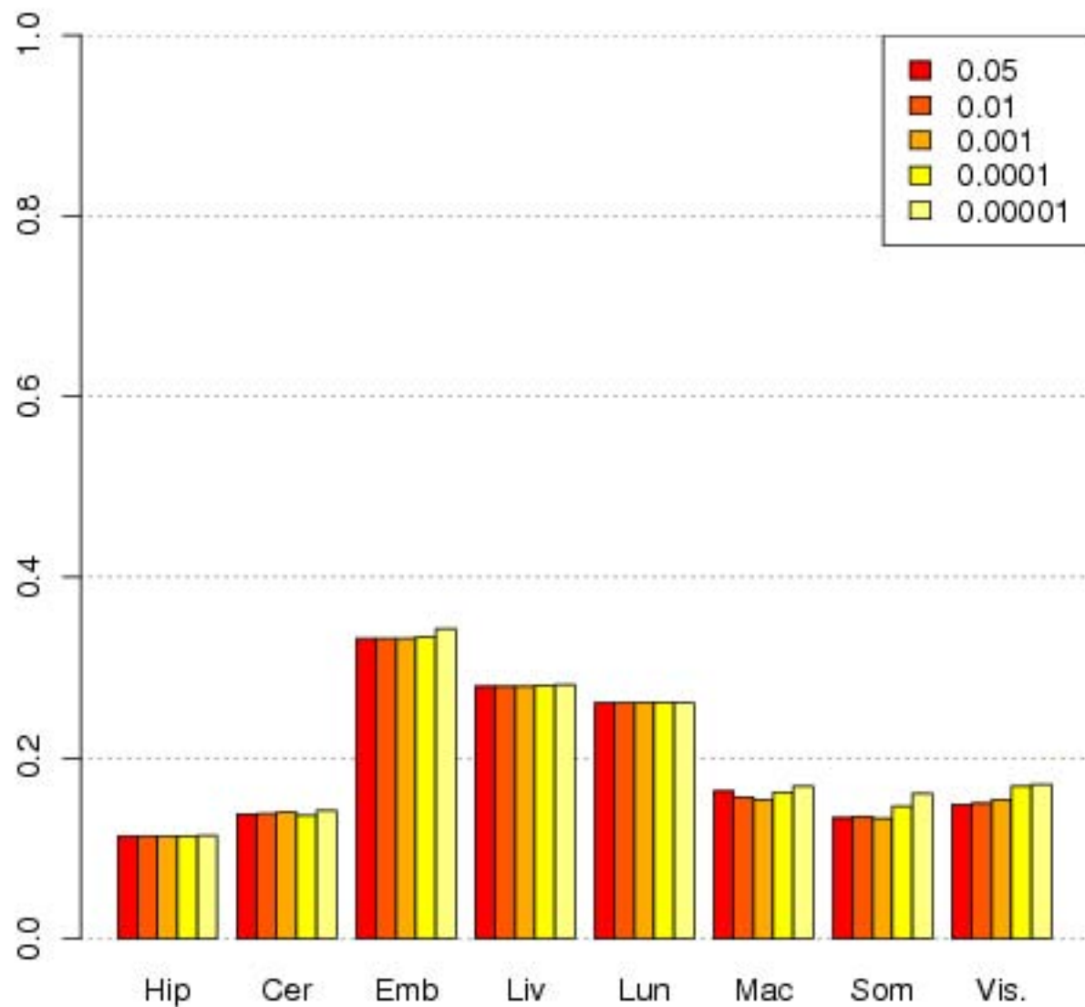
Proportion of TATA-boxes at 80%
