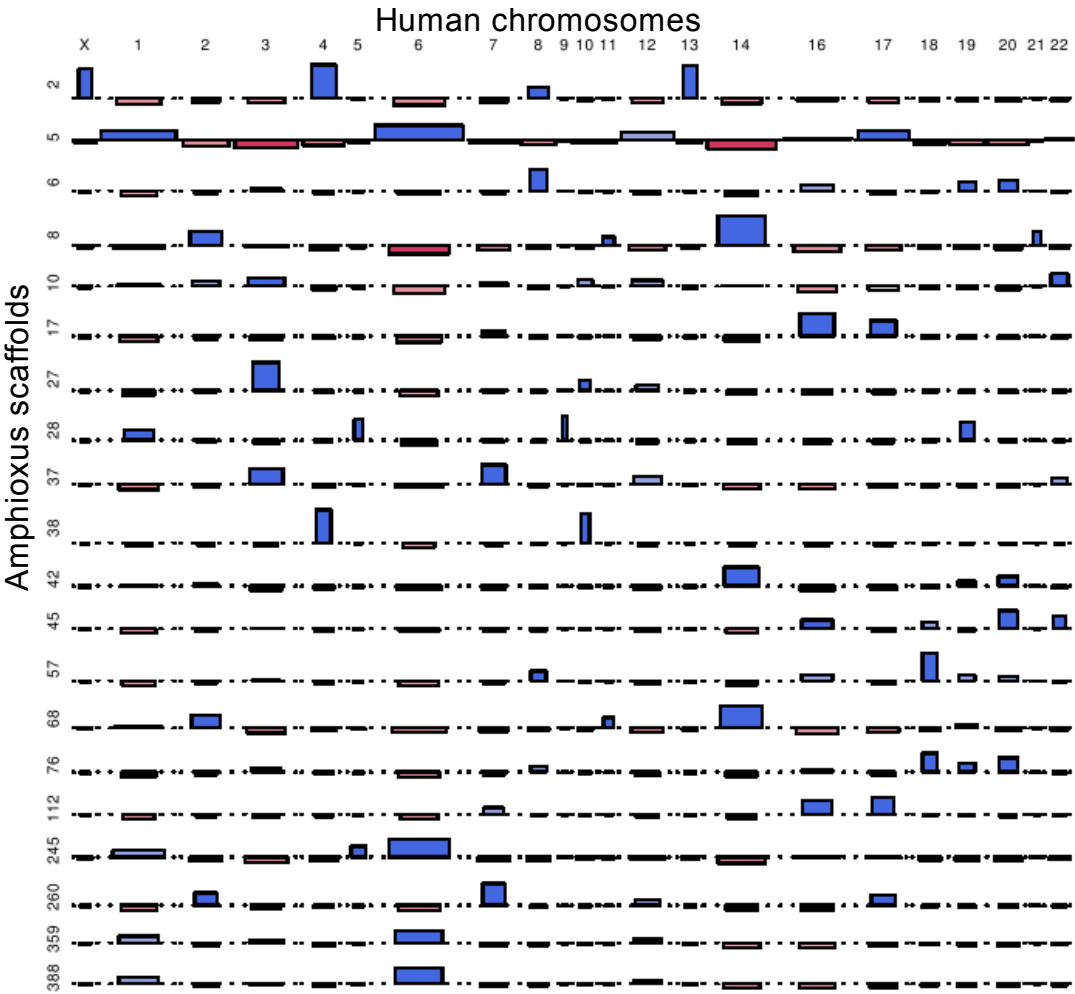
Supplementary Fig. S2. Friendly-Cohen plot of the human chromosomes vs. the largest amphioxus scaffolds.
