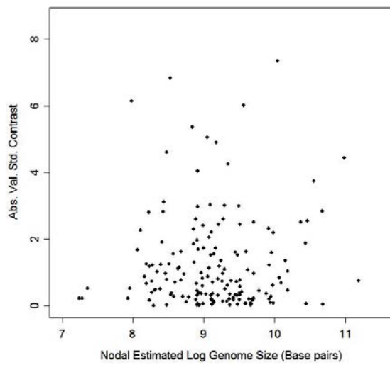
Supplementary Figure 2: A priori \text{Log}_{10} transformation of genome size removes the proportional effect of genome size on the rate of genome size evolution, even when a chronogram estimated from the 18S rDNA tree is used for the contrast calculation.
