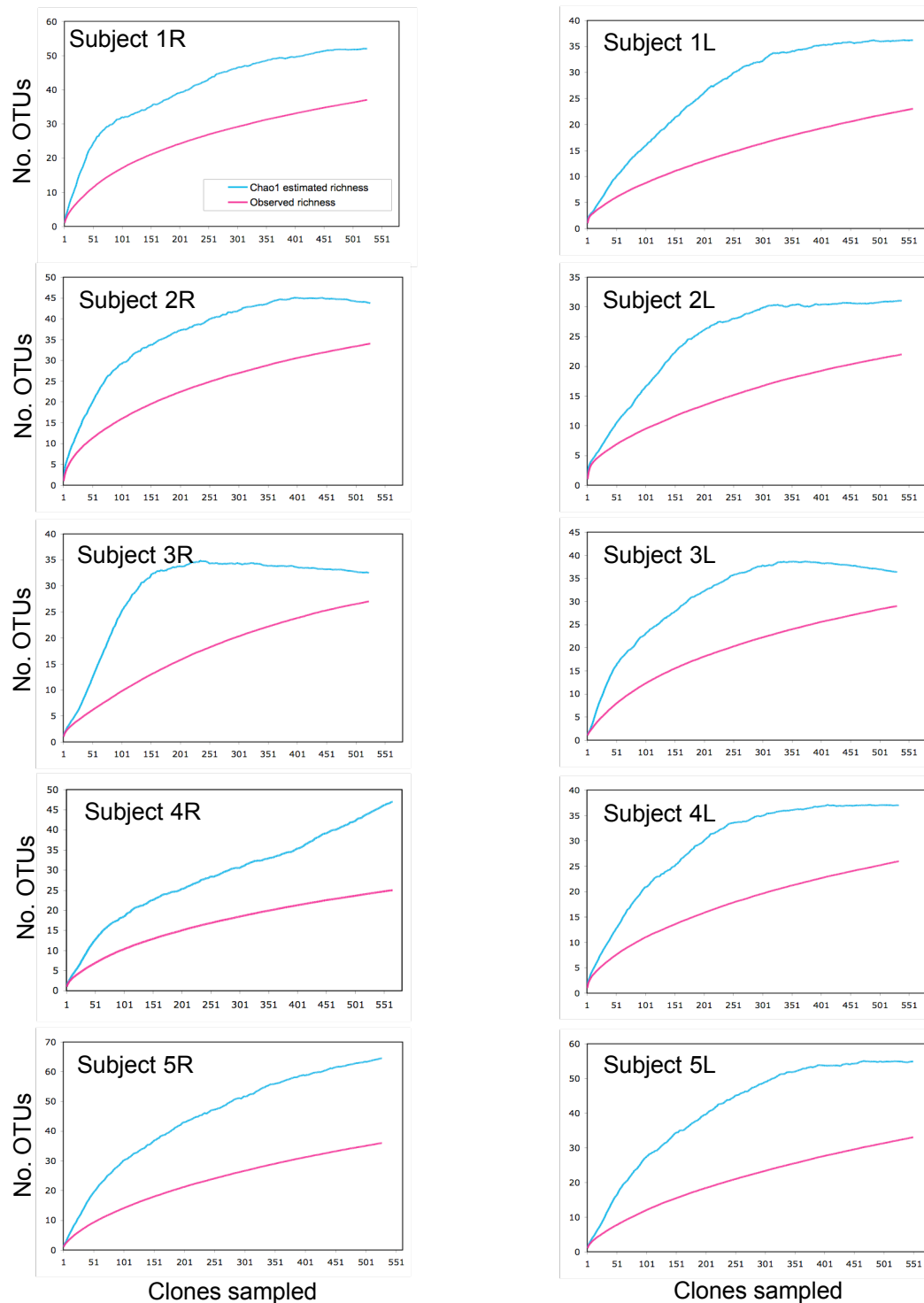
Figure S3: Rarefaction curves of observed and estimated (Chao1) OTU richness for each arm of each subject using an OTU threshold of \geq 97\% identity. As more clones are arbitrarily added, observed and estimated OTUs levels off. The gap between observed and estimated richness indicate that if more clones were sampled, richness would likely continue to increase.
