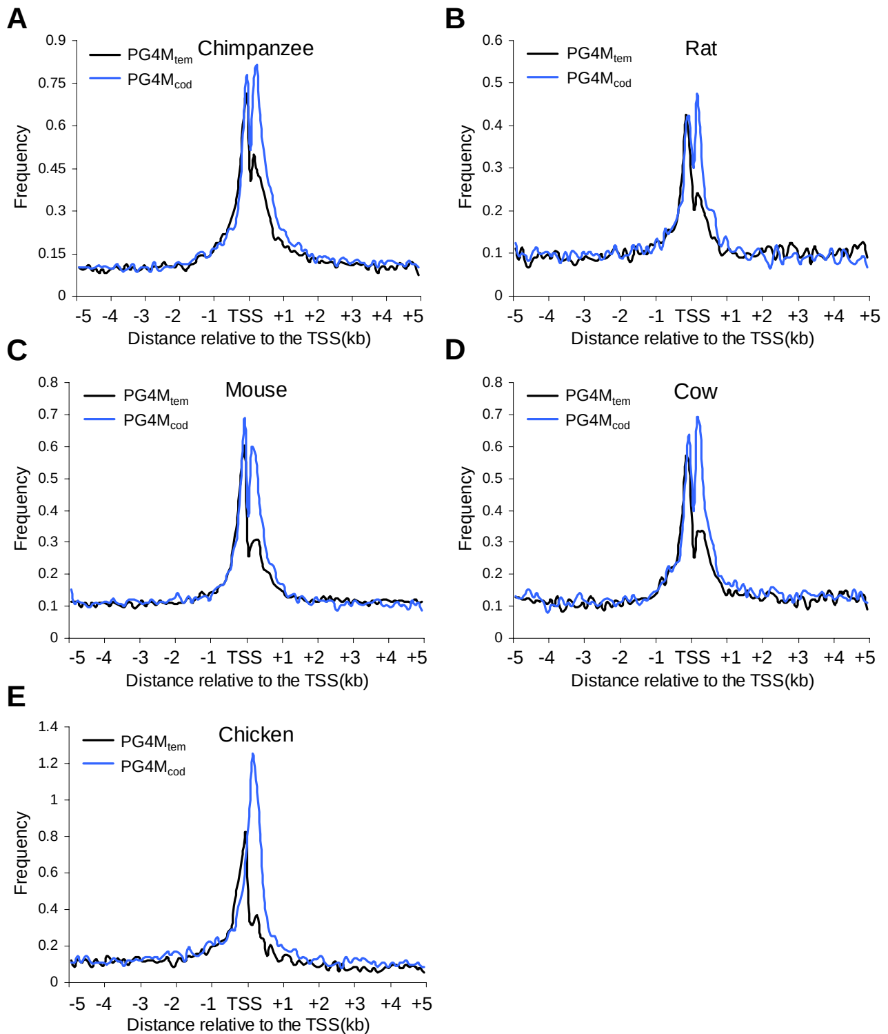
Supplemental Figure S2 Strand asymmetry of PG4M D500 in warm-blooded animals. The frequencies of PG4Ms on the coding (PG4M cod ) and the template (PG4M tem ) strands in the 10 kb TSS-flanking region (TSS \pm 5 kb) of five selected warm-blooded animals are plotted (A–E).
