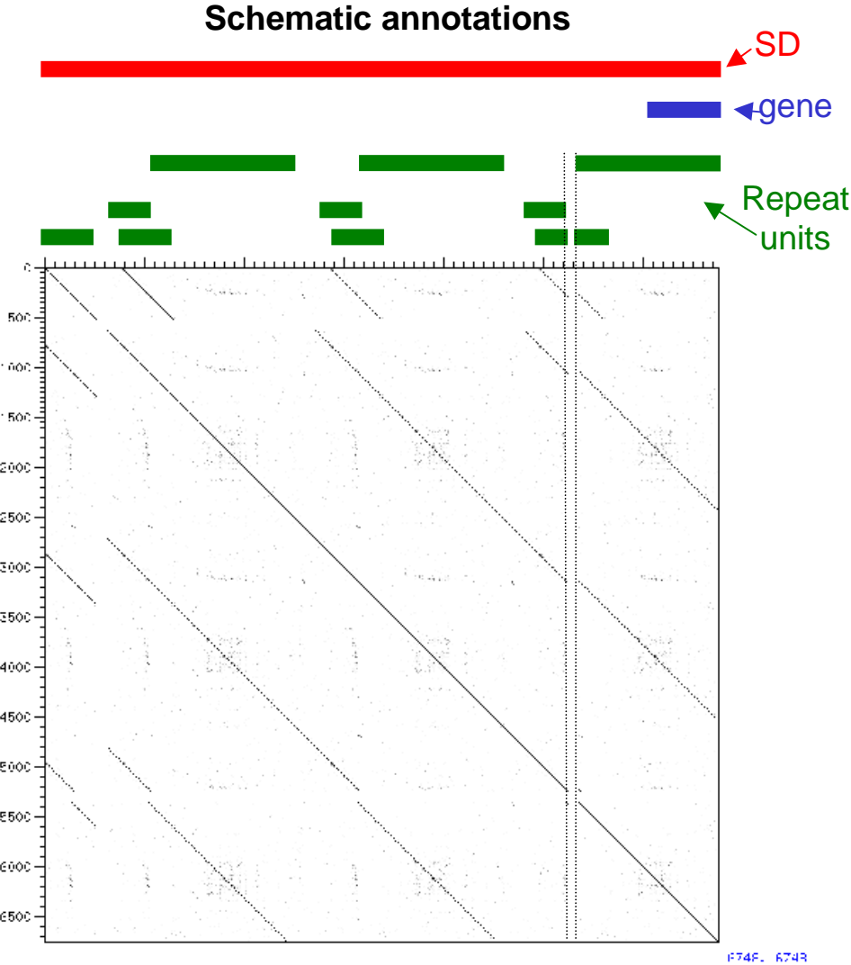
Dotplot of the detected sequence with itself
