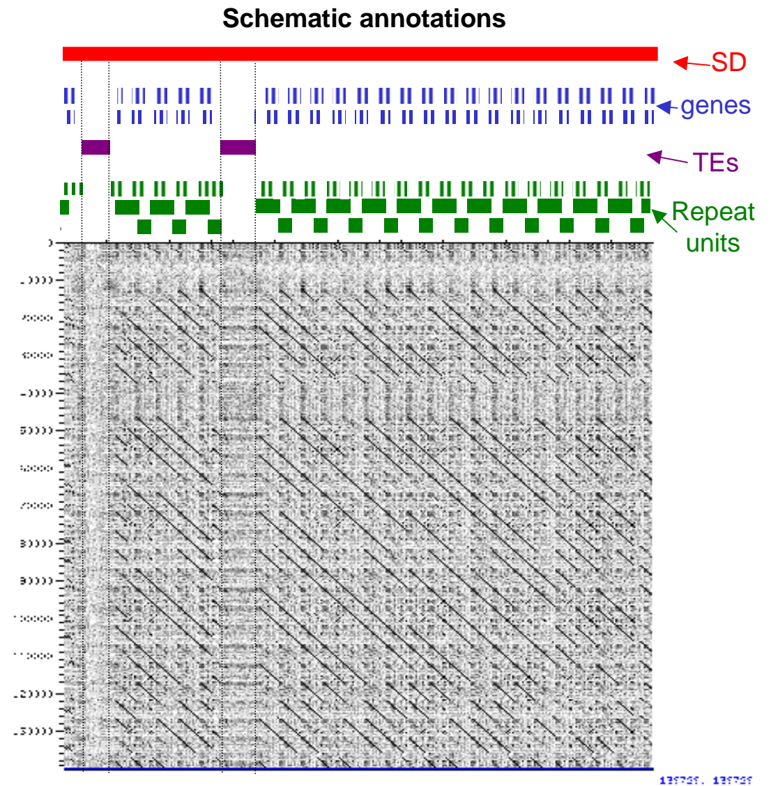
Dotplot of the detected sequence with itself
