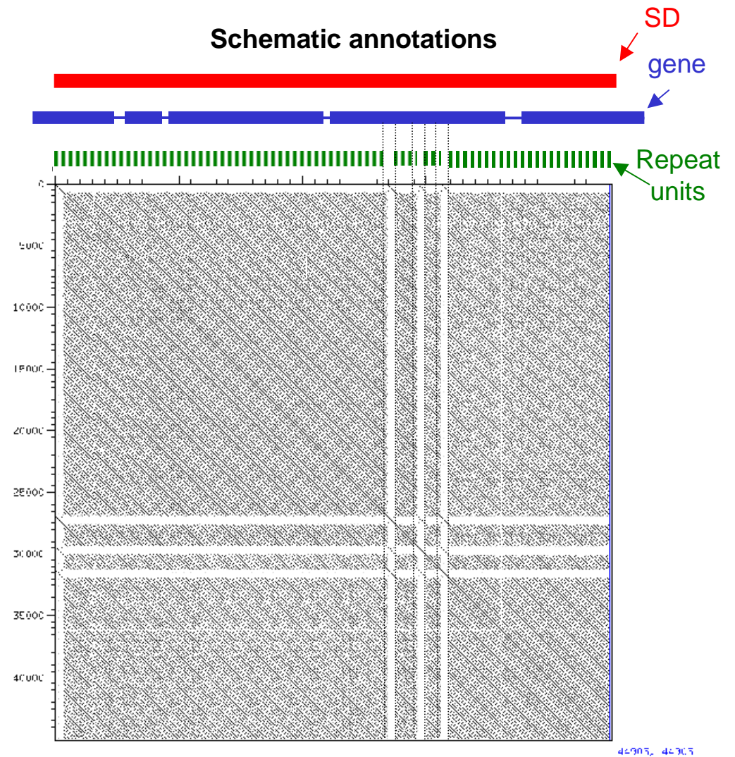
Dotplot of the detected sequence with itself
