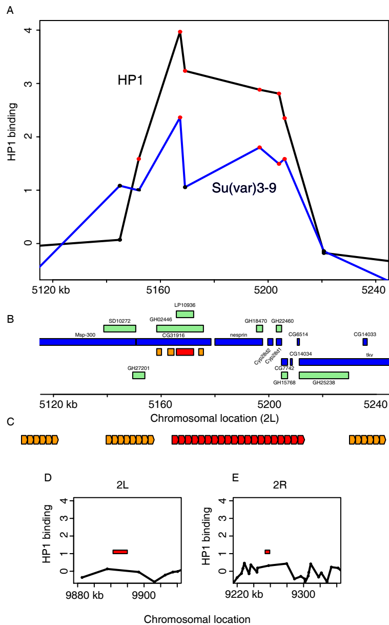
Figure S1: Binding of HP1 and Su(var)3-9 to arrays of tandemly repeated elements. A) Binding pattern of HP1 (black) and Su(var)3-9 (blue). Location of the genes (blue) and microarray cDNAs (green). Red and orange rectangles highlight the location of the repeat arrays. C) Close-up of the tandemly repeated array. Same color indicates the same sequence. D,E) Examples of HP1 binding in the vicinity of two other arrays of tandem repeats.
