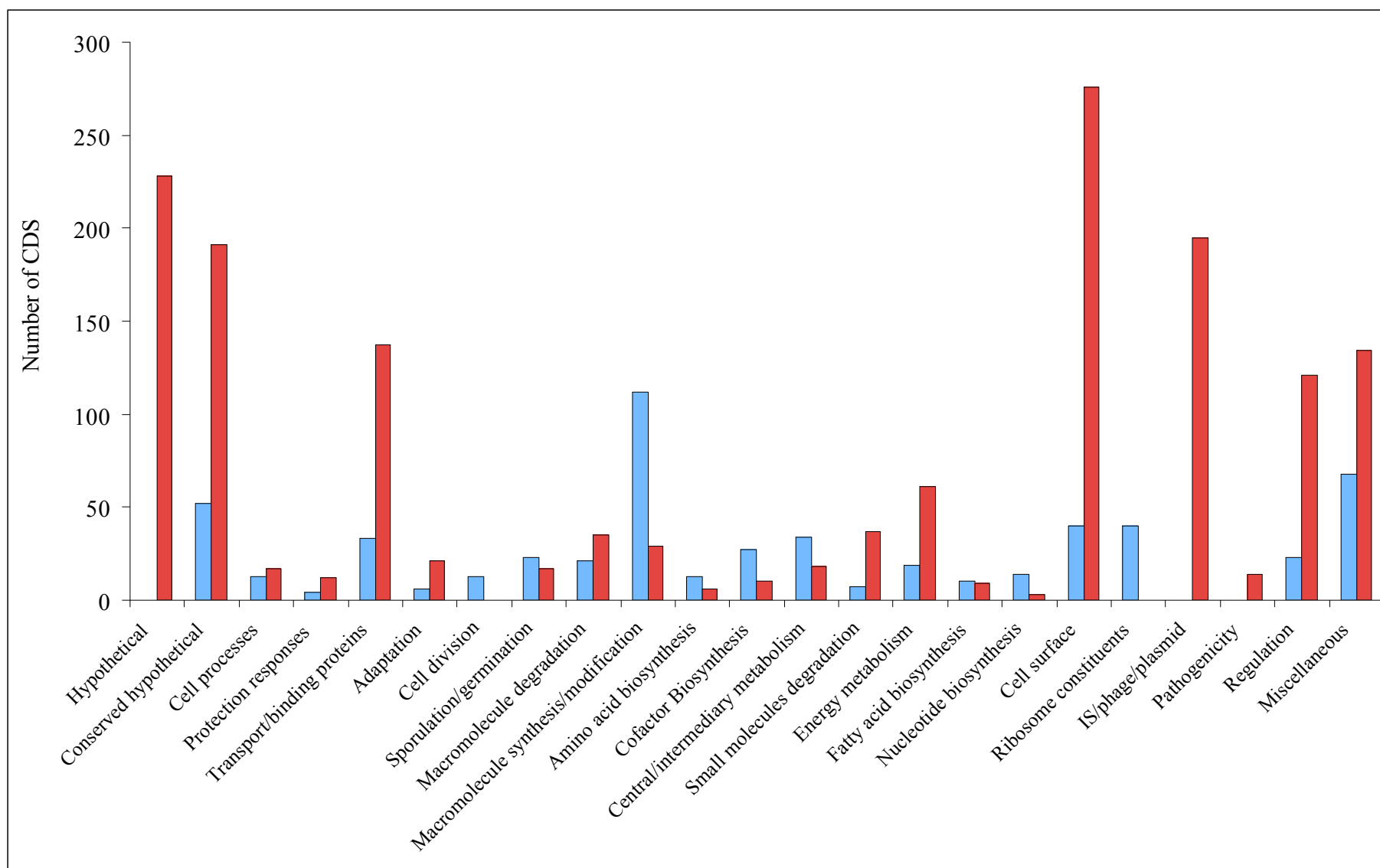
Figure S1. Representation of the distribution by functional categories of the shared (blue) and unique (red) C. botulinum CDSs relative to the sequenced clostridial genomes.
