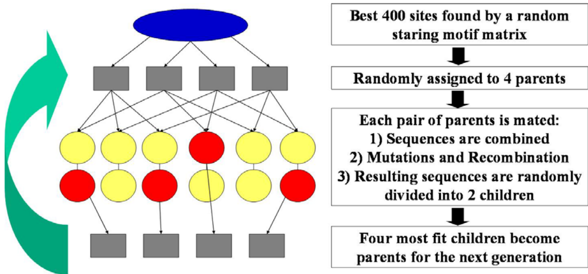
Supplemental Figure 2. Flow chart of the genetic algorithm. Blue oval represents the initial starting motif alignment. Squares represent parents. Circles represent progeny. Red Circles represent the most fit progeny which are selected as parents for the next generation.
