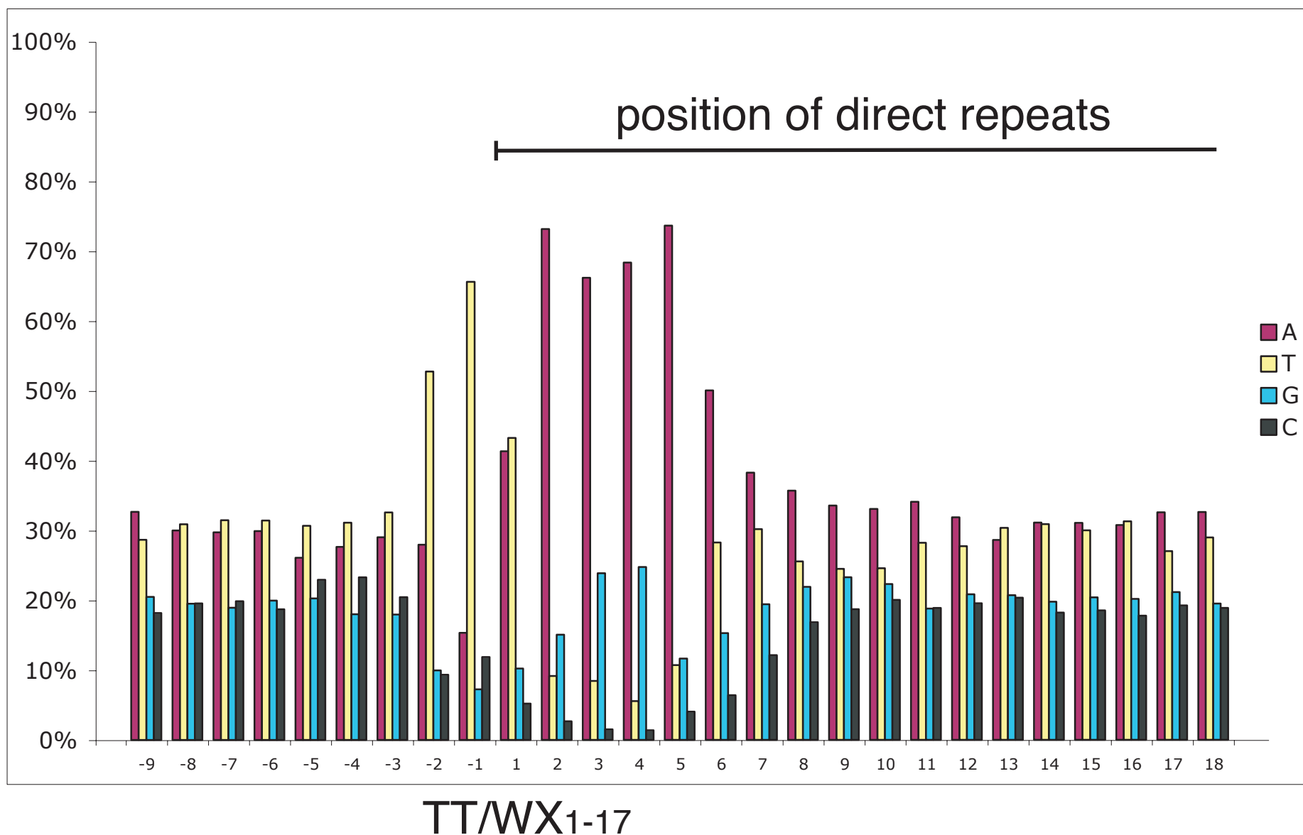
Supplementary Figure 3 online: Percentage nucleotide composition around the integration site for all tRNA-related tailless retropseudogenes Red bars indicate adenine, yellow bars thymine, blue bars guanine, and black bars cytosine. The tailless retropseudogenes integration motifs are shown below the bars.
