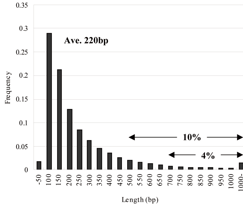
Length ditribution of the putative "homologous" regions in non-genic regions
