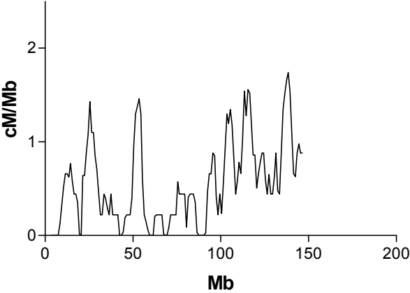
Mouse Chr 5
