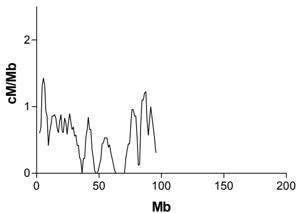
Mouse Chr 16
