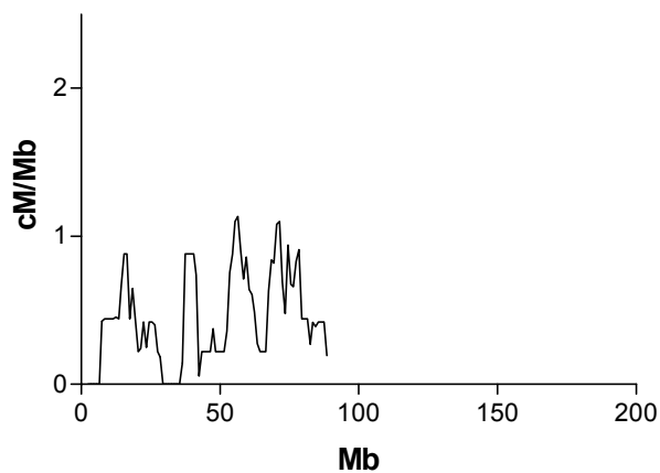
Mouse Chr 18
