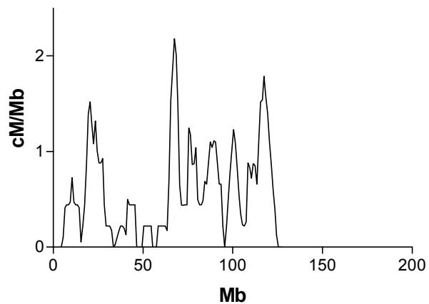
Mouse Chr 10
