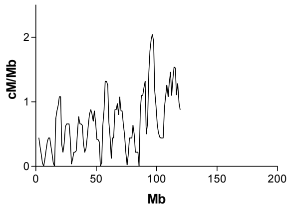
Mouse Chr 11
