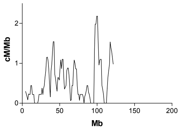
Mouse Chr 9
