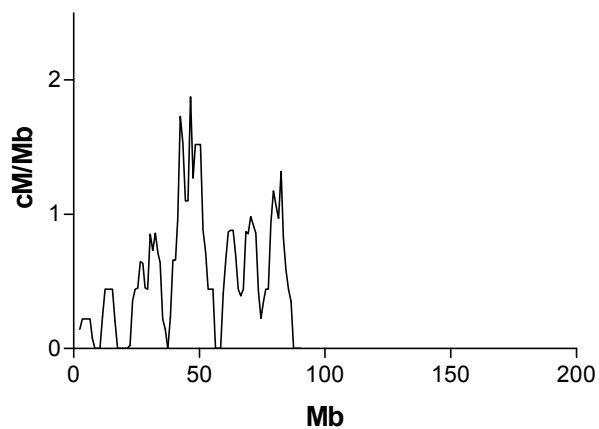
Mouse Chr 17
