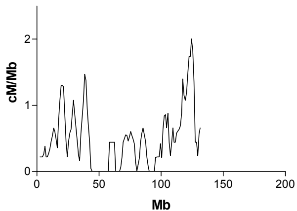
Mouse Chr 7
