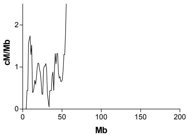
Mouse Chr 19
