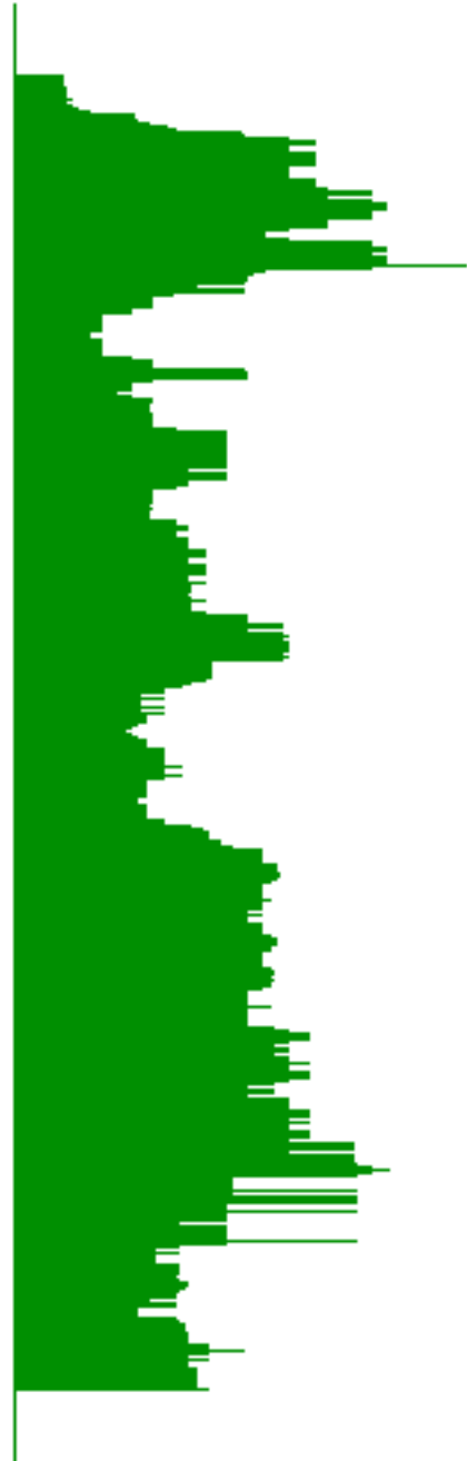
Gene expression
