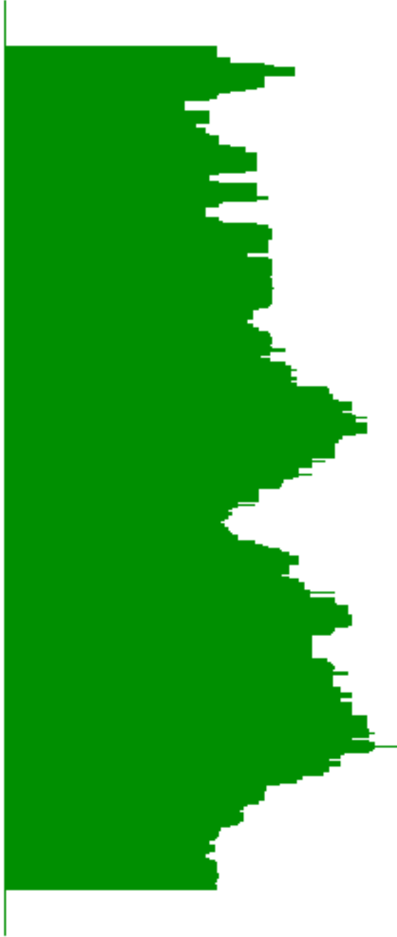
SINE content
