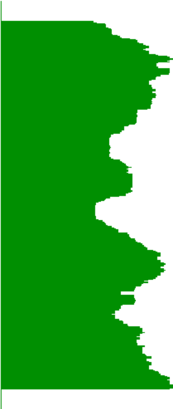
GC content
