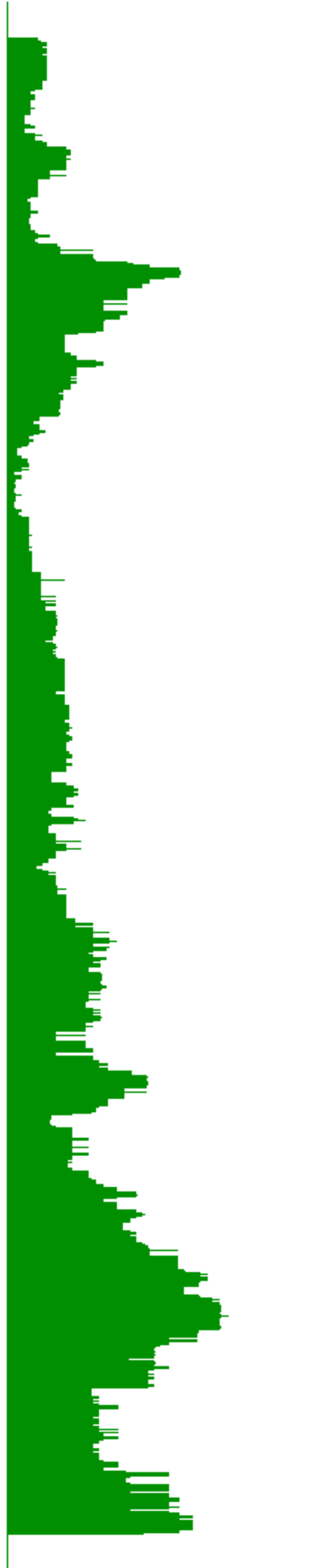
Gene expression
