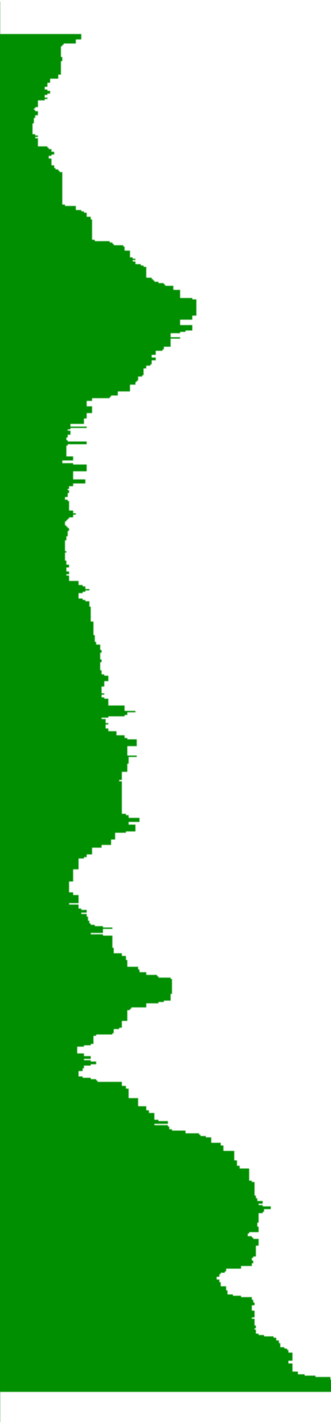
GC content
