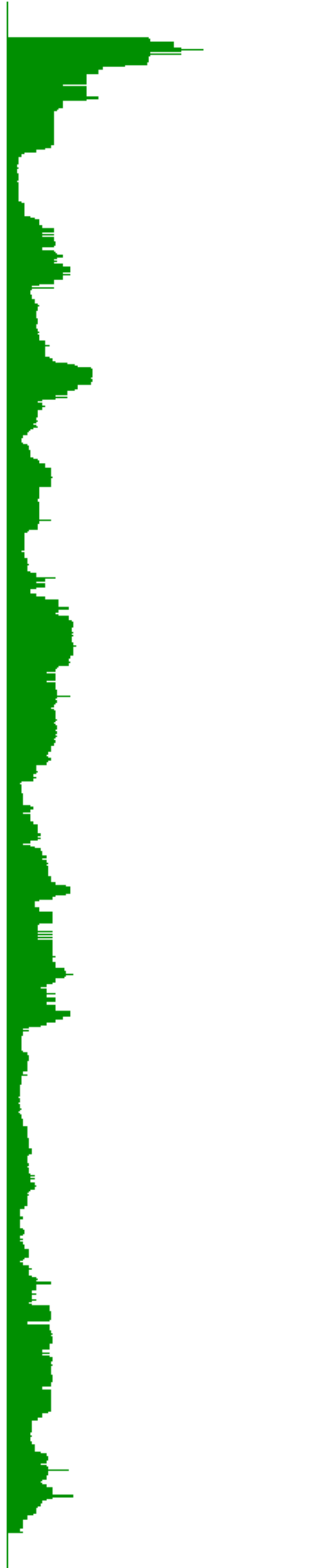
Gene expression
