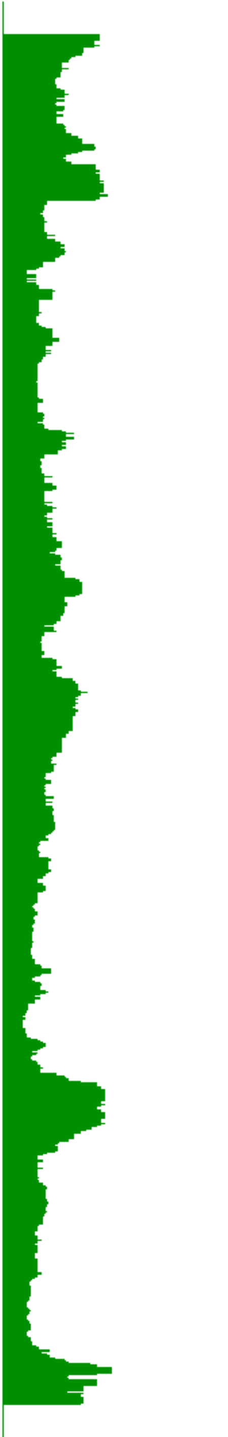
Gene density
