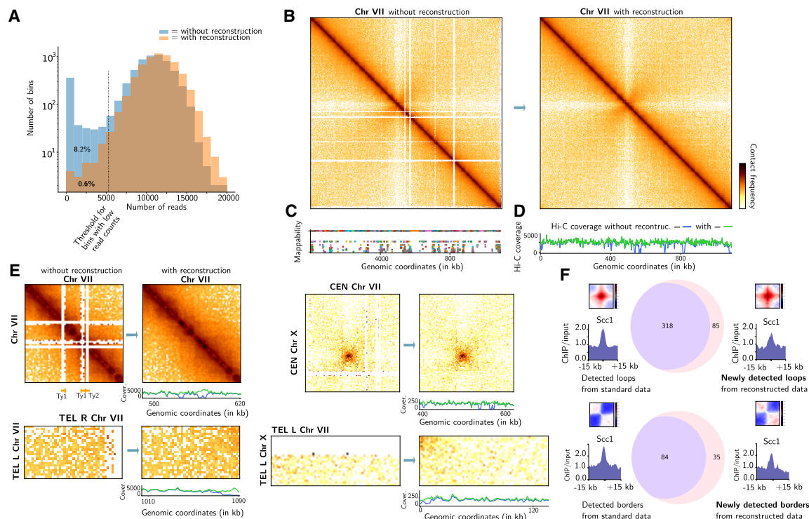
Figure 3. Examples of HiCberg reconstructions in the genome of the model organism S. cerevisiae . (A) Distribution of the number of reads per bin for standard Hi-C experiment in yeast S. cerevisiae without and with HiCberg reconstruction. The threshold used to filter bins with few reads before normalization corresponds to five median absolute deviations below the median log marginal sum and is represented by a dashed line. (B) Chromosome contact map without and with HiCberg reconstruction for Chromosome VII (bin = 2 kb, with normalization) (C) Mappability signal along the Chromosome VII. (D) Hi-C coverage before (green) and after (blue) HiCberg reconstruction. (E) Examples of reconstructions at representative regions: on several yeast transposons (Ty) at Chr VII, between both telomeres TEL-L and TEL-R of Chr VII, between centromeres of Chr VII and Chr X, and between telomeres TEL-L of Chr VII and TEL-L of Chr X with Hi-C coverages without and with reconstruction. (F) Detection of chromosomal loops and borders on data without and with reconstruction. Pileup plots for detected loops and borders for both types of data are shown as well as average signal around anchors of ChIP-seq signal of Scc1, a cohesin subunit.
