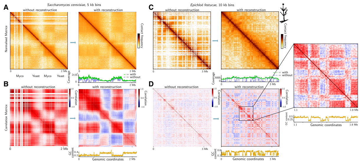
Figure 4. Compartment reconstruction signals by HiCberg. (A) Normalized contact map of the chimeric Chromosome XVI of S. cerevisiae and M. mycoides binned at 5 kb resolution without and with HiCberg reconstruction. The GC content of the sequences and annotations for S. cerevisiae and M. mycoides are shown below the left panel, and the Hi-C coverages before (blue) and after (green) the HiCberg reconstructions are shown below the right panel. (B) Correlation matrices of the chimeric Chromosome XVI of S. cerevisiae and M. mycoides binned at 5 kb resolution without and with reconstruction. The GC content is shown below the map on the right. (C) Normalized contact map of Chromosome 5 of Epichloë festucae binned at 10 kb resolution without and with reconstruction. Hi-C coverages before (blue) and after (green) HiCberg reconstruction are shown below the right panel. (D) Correlation matrices of Chromosome 5 of E. festucae binned at 10 kb resolution without and with reconstruction. The GC content (orange) is shown below the map on the right. A zoom-in of the contact map is shown in relation to the GC content signal below.
