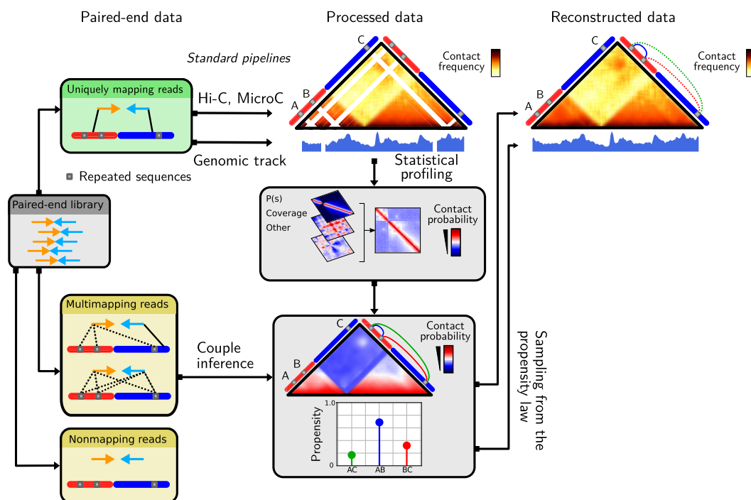
Figure 1. General principles of the Hicberg method for the reconstruction of contact maps and genomic tracks. Read pair reconstruction involves classification into three groups (nonmapping, uniquely mapping, and multimapping reads). The uniquely mapping fraction of reads is used to profile the statistical trends of the data. Several components can be included in the statistical model: chromatin polymeric behavior P(s) , genome coverage, and others. The statistical model computes the propensities for each potential contact to occur, and the propensity distribution is built. For each ambiguous pair, a single possibility is then chosen according to the propensity distribution.
