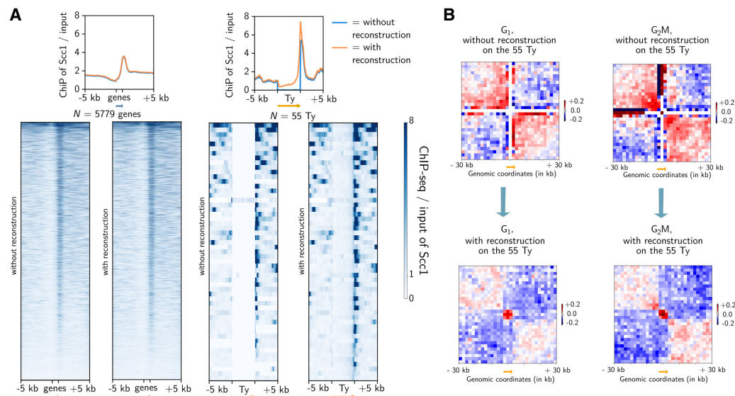
Figure 7. Averaged signal of cohesin occupancy and agglomerated contact plot of the transposons (Ty) in the yeast S. cerevisiae genome. (A) Averaged signal of cohesin occupancy (ChIP-seq of Scc1) at genes and at Ty elements without and with Hicberg reconstruction in the yeast S. cerevisiae in the G 2 /M phases of the cell cycle. (B) Agglomerated contact plots of Ty in the G 1 and G 2 /M phases of the cell cycle without and with Hicberg reconstruction in the yeast S. cerevisiae .
