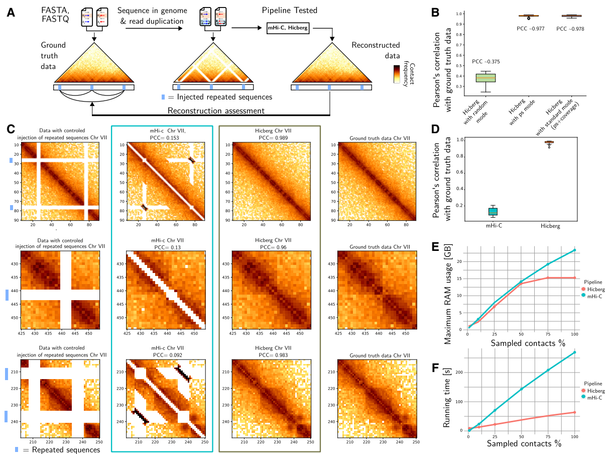
Figure 2. In silico bench testing strategy for assessing the quality of HiCberg reconstructions. (A) Controlled ambiguity is injected by duplicating sequences and selected reads in the FASTA and FASTQ files at chosen positions. This ambiguity is then confronted with HiCberg reconstruction after profiling and statistical inference. The ground truth and the data reconstructed through HiCberg are compared to assess the quality of the proposed reconstruction via the Pearson's correlation coefficient (PCC). (B) Comparison of the HiCberg method with three different modes of determination of contact probabilities: random mode (uniform distribution between the different contacts) and P(s) mode using the frequency of contact in function of genomic distance, with standard mode using in addition the genomic coverage. (C) Comparison of the mHi-C and HiCberg methods evaluated using the benchmark shown for three different representative regions: from left to right, contact map from data with controlled injection of repeated elements (blue boxes), with data reconstructed with mHi-C, with data reconstructed with HiCberg, and from ground-truth data. PCCs with the ground-truth data are given for mHi-C and HiCberg reconstructions. (D) Comparison of the mHi-C and HiCberg methods evaluated using the benchmark. The box plot shows the distribution of 24 comparisons using the PCC between the reconstructed region and the same region derived from the ground-truth data. (E) Memory usage of both HiCberg and mHi-C according to the subsampling of Hi-C data of S. cerevisiae from 5% to 100% of the 47 million pairs of reads of the data. (F) Runtime of both HiCberg and mHi-C according to the subsampling of Hi-C data of S. cerevisiae from 5% to 100% of the 47 million pairs of reads in the data.
