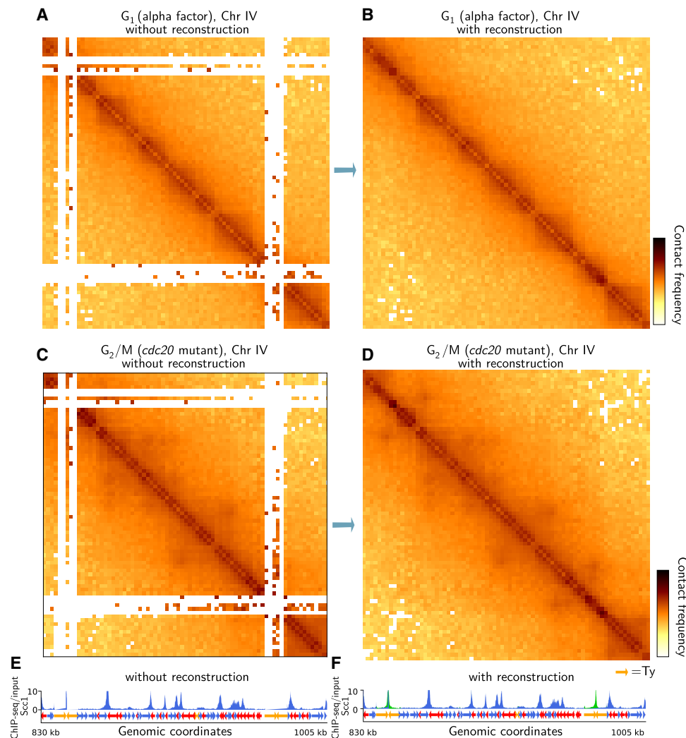
Figure 6. Yeast transposons can be associated with the positioning of cohesin loops in the S. cerevisiae genome. (A,B) Zoomed view of the contact map of Chromosome IV of S. cerevisiae without and with Hicberg reconstruction; bin=2 kb in a population synchronized in the G 1 phase (W303 strain) (data from Piazza et al. 2021). (C,D) Zoomed contact map of Chromosome IV of S. cerevisiae without and with Hicberg reconstruction in a population synchronized in the G 2 /M phase (W303 strain, cdc20 mutant) (data from Piazza et al. 2021). (E,F) Cohesin occupancy signal from ChIP-seq of Scc1 in the G 2 /M phase without and with Hicberg reconstruction. The forward and reverse genes are represented by blue and red arrows, respectively. Retrotransposons are represented by orange arrows. The black triangles point to chromosomal loops that are only visible with Hicberg reconstruction and are associated with cohesin occupancy peaks (Scc1) at convergent transposons.
