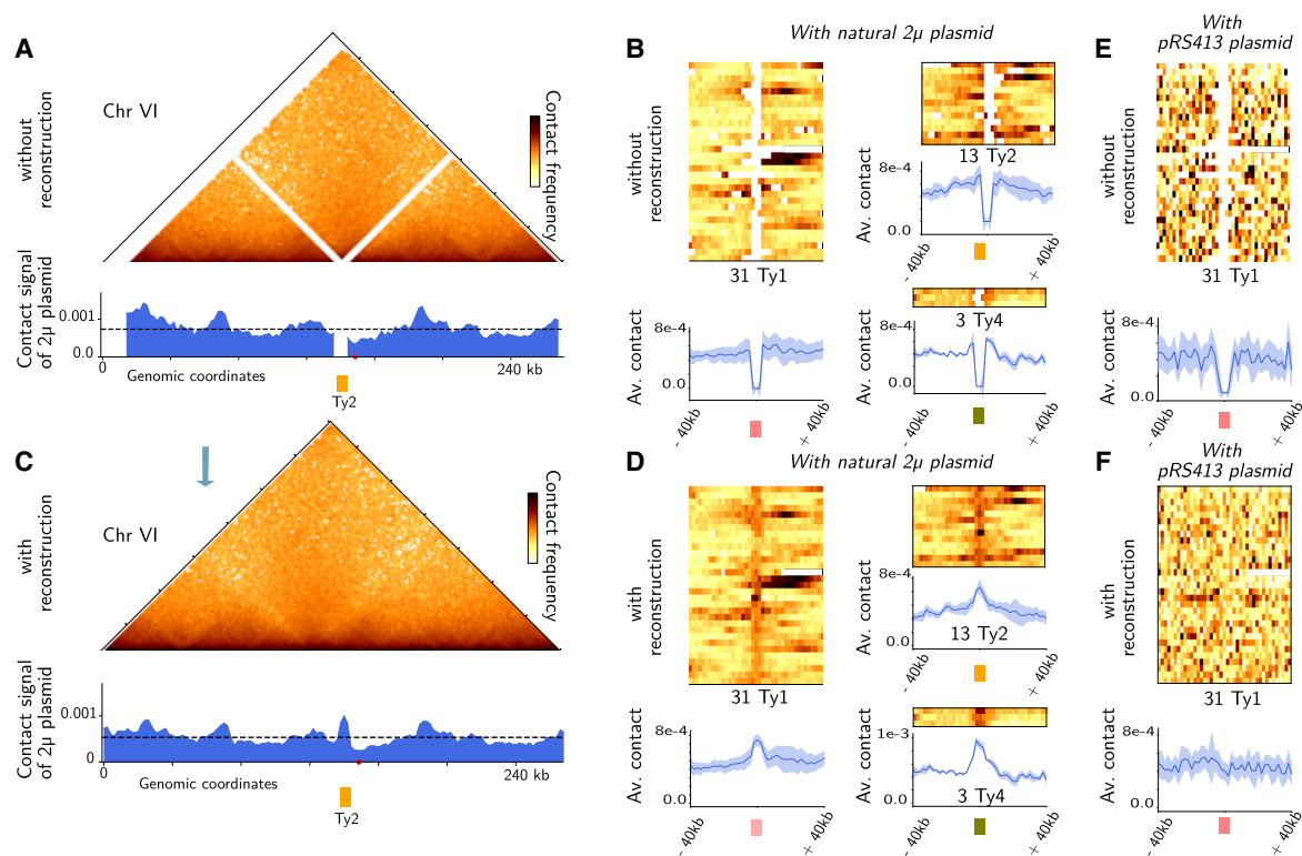
Figure 5. Parasitic 2 \mu plasmid shows contact enrichment with yeast transposons. (A) Contact map of Chromosome VI of S. cerevisiae without reconstruction; bin = 2 kb in the asynchronous population (BY4741 strain). Below is the contact signal of the 2 \mu plasmid along Chromosome VI without reconstruction. (B) Heatmap representing the contact signals of the 2 \mu plasmid with three different families of yeast transposons: Ty1 (31 elements), Ty2 (13 elements), and Ty4 (3 elements) without reconstruction. Below is the averaged signal (in blue) over the different elements of each family. (C) Contact map of Chromosome VI of S. cerevisiae with reconstruction, bin = 2 kb. Below is the contact signal of the 2 \mu plasmid along Chromosome VI with reconstruction. (D) Heatmap representing the contact signals of the 2 \mu plasmid with three different families of yeast transposons: Ty1, Ty2, and Ty4 with reconstruction. Below is the averaged signal summed over the different elements of each family. (E) Heatmap representing the contact signals of the pRS413 plasmid sequence with Ty1 elements without reconstruction. Below is the averaged signal over the different elements for the Ty1 family. (F) Heatmap representing the contact signals of the pRS413 plasmid sequence with Ty1 elements with reconstruction. Below is the averaged signal summed over the different elements of the Ty1 family.
