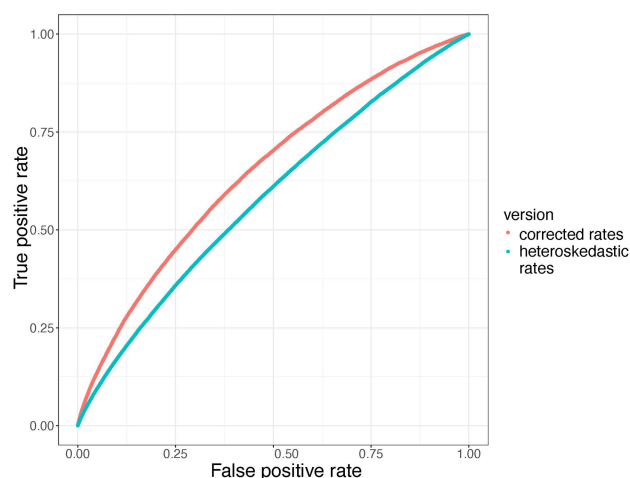
Figure 3. Removal of heteroskedasticity improves ERC predictive power. Receiver operator characteristic (ROC) curves contrasting true-positive and false-positive rates demonstrate higher power in ERC2.0 values calculated using corrected rates (red curve; AUC = 0.652) compared with ERC1.0 values using uncorrected, heteroskedastic rates (blue curve; AUC = 0.581). The true-positive set are interactions from STRING with combined scores that are more than 700. ERC scores were calculated on a phylogeny of 18 yeast species.
