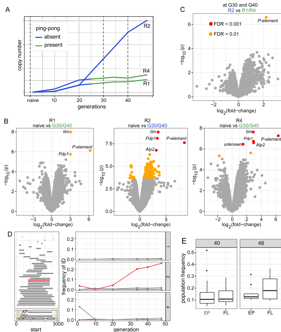
Figure 5: Differences among replicates with (R1,R4) and without (R2) P-element ping-pong. A) Schematic overview of the RNA-seq samples used for identifying genes differentially expressed among samples with (green) and without P-element ping-pong (blue). B) Volcano plots highlighting expression differences for TEs and D. erecta transcripts between naïve flies and invaded flies (generations 30 and 40). Data are shown for all three replicates (R1, R2, R4). C) Volcano plot highlighting expression differences between replicates with and without P-element ping-pong at generations 30 and 40. D) Overview of P-element insertions with internal deletions in the experimental populations (left panel). The lower left panel shows the composition of the P-element and the deleted regions of D50 and the KP-element . The DNA-binding domain (orange) and regions necessary for mobilizing the P-element (green) are indicated (Majumdar and Rio, 2015). The right panel shows the frequency of the IDs (relative to all P-element insertions) in the three replicates. Note that the EP-element (red), i.e. a P-element variant with deletion of a similar region than for the KP-element , is increasing in frequency in replicate 2 but not in the other replicates. E) Population frequency of EP-element insertions and the full-length (FL) insertions of the P-element in replicate 2 at generations 40 and 48.
