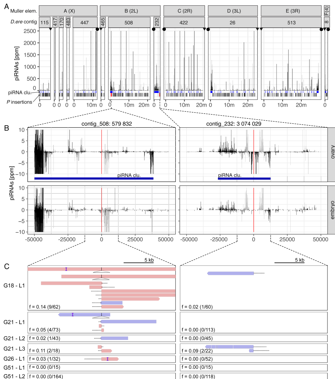
Figure 3: At least two P-element insertions in germline clusters are present in replicate 2 at early stages of the invasion (generations 18-26). A) Overview of ambiguously (light grey) and unambiguously (black) mapping piRNA in 1kb windows along the 12 largest contigs of the D. erecta assembly. The corresponding Muller element and the likely direction of the telomere (triangle) and the centromere (circle) are shown. At the bottom we show the positions of the annotated piRNA clusters (blue) of P-element insertions outside (black) and inside of piRNA clusters (red bold; solely insertions in replicate 2 at generations \leq 26 supported by at least two long-reads are shown). B) Abundance of piRNAs in a 100kb window around the two insertions in piRNA clusters for both ovaries and embryos. Sense piRNAs are on the positive y-axis and antisense piRNAs on the negative y-axis. Ambiguously (light grey) and unambiguously (black) mapped reads are shown. C) Support of the P-element insertions by long reads at different generations ( Gxx ) and in different sequencing libraries ( Lx ). Sense reads are shown in red, and antisense reads are in blue. Regions of the reads aligning to the P-element are shown as dashed lines (true to scale). For each library, we indicate the population frequency of the P-element insertion ( f ), the number of reads supporting the insertion and coverage at the insertion site (in brackets: reads/coverage). Note that both insertions are likely full-length P-element insertions (almost the complete P-element is covered by some reads) and that both insertions are likely lost (or at very low frequency) by generation 51.
