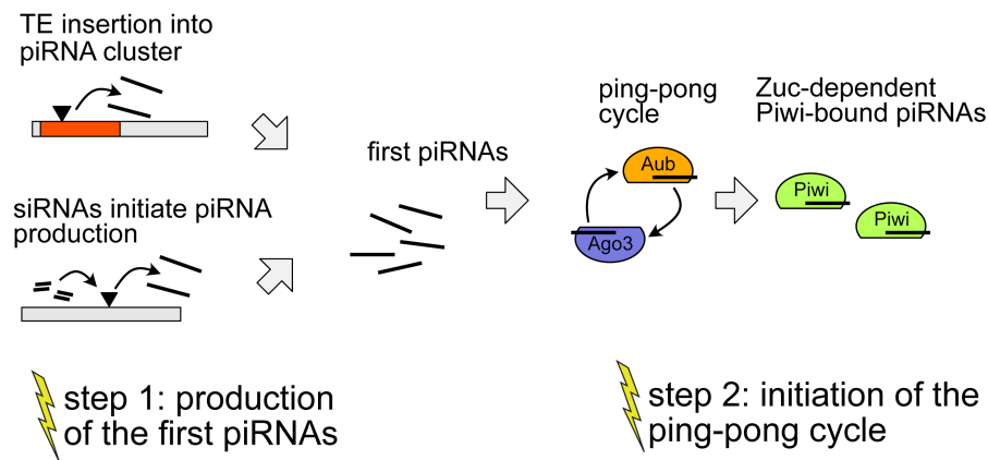
Figure 7: Two steps may be necessary to activate the host defense against an invading TE. According to the prevailing view, i.e. the trap model, a TE insertion into a piRNA cluster is sufficient to trigger the host control over an invading TE. In our updated model, the two-step model, we propose that silencing of an invading TE requires two steps: i) the generation of some first piRNAs and ii) the initiation of the ping-pong cycle. Yellow flashes indicate necessary events for establishing the host control
