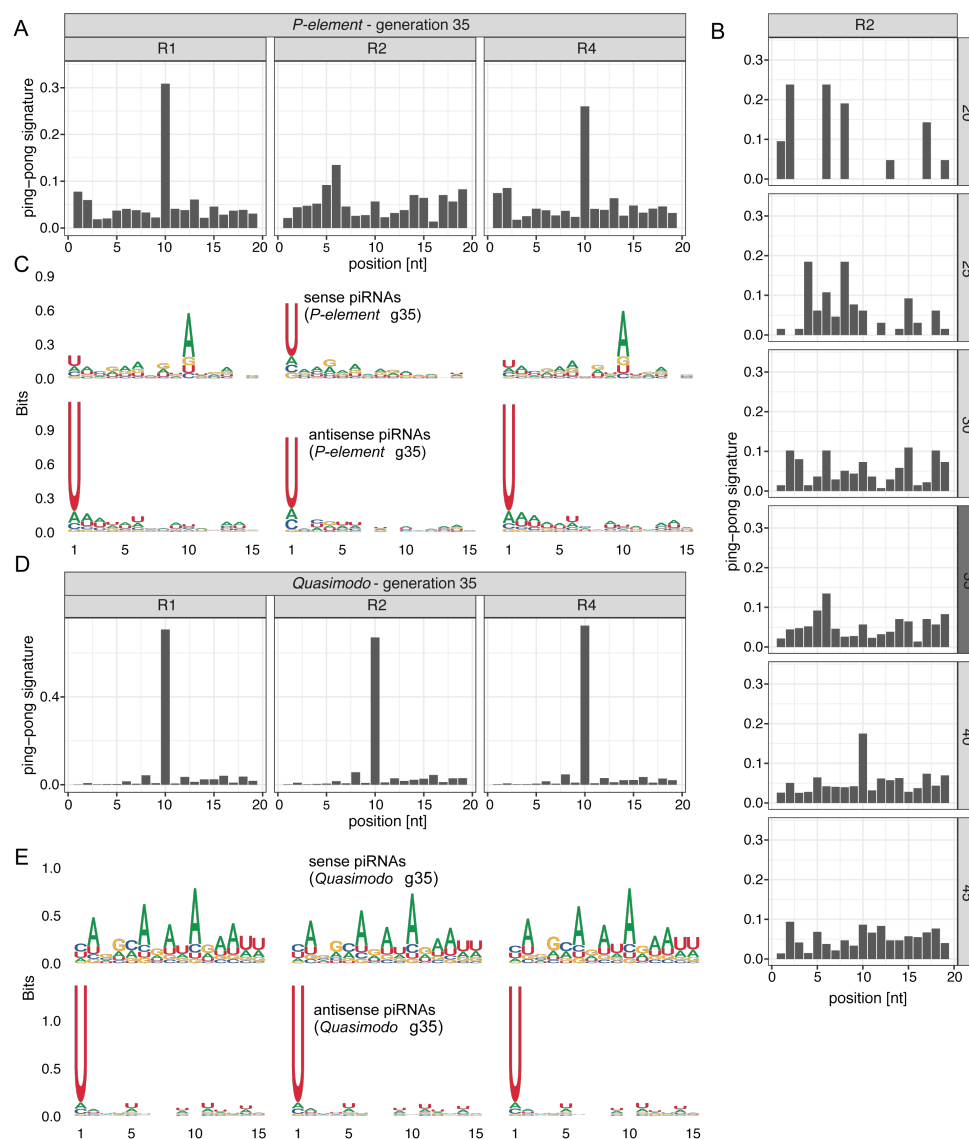
Figure 2: P-element ping-pong is inactive in replicate 2. A) The ping-pong signature (peak at position 10) of the P-element in ovaries at generation 35. Note that the ping-pong signature is missing in replicate 2. B) The ping-pong signature of the P-element in replicate 2. Data are shown for all generations with sufficient piRNAs. Small RNA extracted from ovaries and whole flies are shown in dark and light grey, respectively. C) Motifs of sense and antisense piRNAs (23-29nt) complementary to the P-element in ovaries at generation 35. Sense piRNAs in replicate 2 do not show an A-bias at position 10. D) Quasimodo displays a pronounced ping-pong signature in all replicates (ovaries, generation 35). E) Motifs of sense and antisense piRNAs of Quasimodo (ovaries, generation 35).
