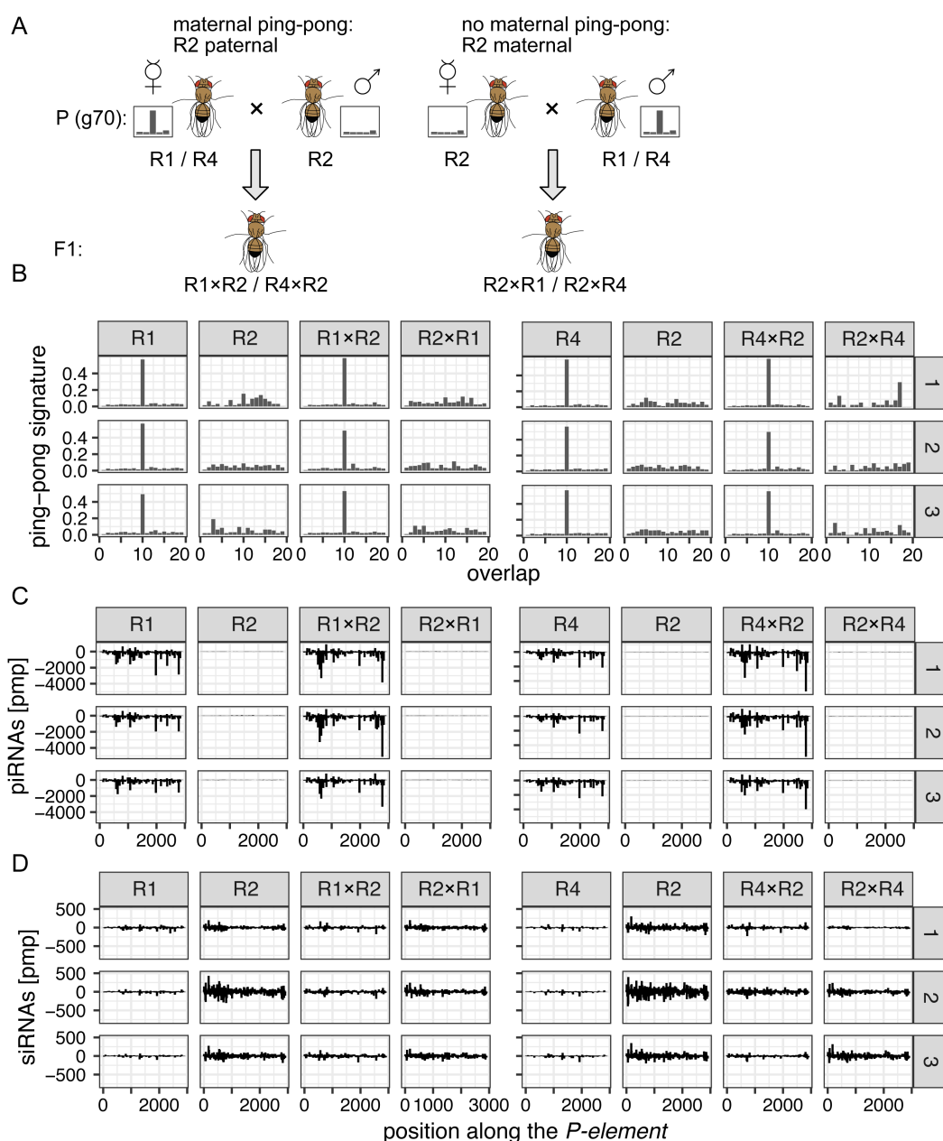
Figure 6: Maternally transmitted factors (possibly small RNAs) and not the genomic composition, are responsible for the absence of P-element ping-pong in replicate 2. A) Crossing scheme for testing the influence of maternal piRNAs. We performed reciprocal crosses among replicates with (R1, R4) and without (R2) ping-pong signature for the P-element . Note that in the F1 offspring of the reciprocal crosses (e.g.: R1×R2 vs R2×R1), the genomic background is largely identical, while the composition of the maternally deposited piRNAs differs. The flies for this experiment were sampled around generation 70 from the experimental populations B) Ping-pong signatures for the P-element in all three replicates (R1, R2, R4) and in the F1 offspring of the reciprocal crosses among the replicates (e.g. R1×R2: R1-female × R2-male). Small RNA was extracted from whole female flies, and three sub-replicates (right panel) were used for each sample. C) Distribution of piRNAs (23-29nt) in the three replicates and the F1 offspring. D) Distribution of siRNAs (20-22nt) in the three replicates and the F1 offspring.
