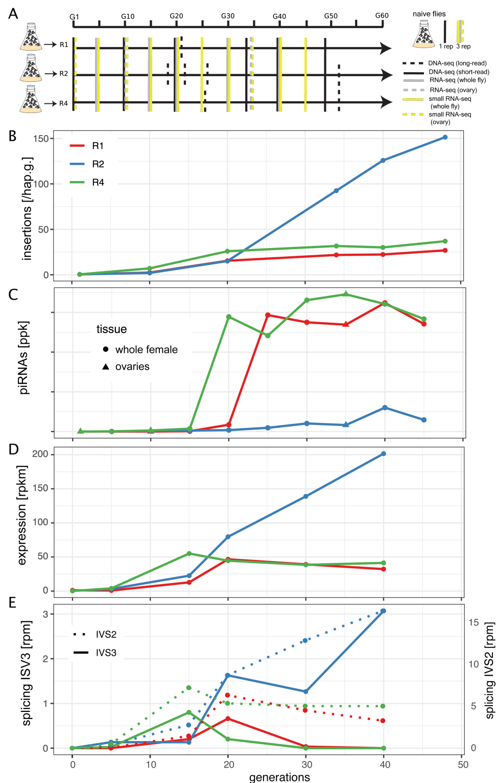
Figure 1: Invasion dynamics of the P-element in experimental D. erecta populations. Data are shown for three replicate populations (R1, R2, R4). A) Overview of the experiment and the sequenced samples. B) Insertions per haploid genome (hap.g.) during the invasion. C) Abundance of piRNAs complementary to the P-element [ppk: P-element piRNAs per 1000 piRNAs]. D) Sense expression of the P-element in whole female flies. Naïve flies are shown at generation zero. E) Splicing of the second (IVS2) and the third (IVS3) intron of the P-element . Naïve flies are shown at generation zero [rpm spliced reads per million mapped reads].
