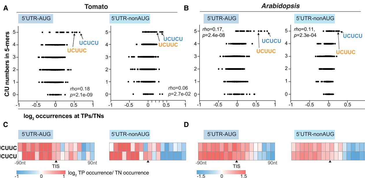
Figure 4. Characterization of putative RNA cis -elements predictive of plant TISs. (A,B) Relationship between the number of C/Us (y-axis) and the enrichment of sequence occurrence (x-axis) for all 5-mers in the tomato (A) and Arabidopsis (B) 5' UTR–AUG and 5' UTR–nonAUG TIS groups. The enrichment is represented as the \log_2 ratio of median sequence occurrence between TPs and TNs in the 200-bp regions centered on TIS sites. Rho indicates Spearman's rank correlation coefficient. (C,D) As described in Figure 3C, but for the enrichment of putative RNA cis -elements in the tomato (C) and Arabidopsis (D) 5' UTR TIS groups. The putative “UCUUC” and “UCUCU” elements with the highest importance score and with the highest enrichment, which are indicated by arrows and highlighted in blue and orange in C,D, are shown.
