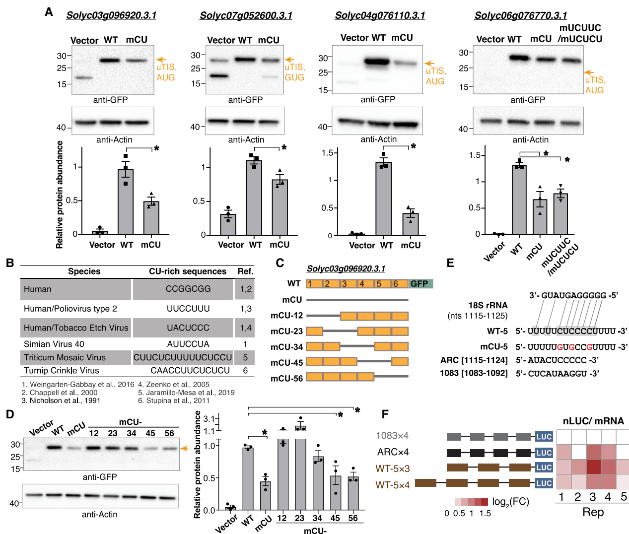
Figure 5. Mutation of CU-rich sequences on plant cellular mRNAs attenuated the TIS activities. (A) Immunoblotting analyses of proteins with translation initiated from the TISs indicated in Supplemental Figure S8 (orange arrows) and with translation driven by the upstream 100-nt wild-type (WT) sequence or sequences with mutations of CU tracts (mCU) or UCUUC/UCUCU (mUCUUC/mUCUCU) sites. Proteins were expressed in Nicotiana benthamiana (tobacco) leaves using the Agrobacterium -mediated transient expression system. Vector indicates tobacco leaves infiltrated with agrobacteria containing the expression vector (i.e., the GFP or FLAG-containing plasmid without a target gene sequence). (Bottom) The protein abundance of the reporter genes relative to actin for three biological repeats (dots) and the corresponding means and standard errors are shown. (B) The known CU-rich sequences found on human transcripts and on plant and animal viral mRNAs promote translation efficiency as reported in the indicated literature. (C) Illustration of swapping the WT (orange box) and the CU-mutated (mCU; gray line) sequences for the TIS-upstream region of a 5' UTR-AUG TIS of Solyc03g096920.3.1 examined in A. The TIS-upstream region was divided into six subregions (indicated in Supplemental Fig. S8A) to generate distinct mCU mutants with indicated CU-mutated regions fused with the GFP reporter gene as described in A. (D) As described in A, but for the protein of the mCU mutants as indicated in C. (E) The putative binding site on WT sequences (shaded), but not on CU-mutated ones, to the plant 18S rRNA (solid and dashed lines). The sequences of the plant 18S rRNA at positions nt 1115 to 1125 and the WT sequence or sequence with mutations of CT tracts (red) in the fifth region indicated in C are shown. (*) P -values < 0.05, which is derived from one-way ANOVA test, representing the significant difference between WT and the samples with CU sequence mutations. (F) Heatmap shows the nLUC/ mRNA ratio for five biological replicates: 1083 × 4 and ARC × 4 denote negative and positive controls with four copies of 1083 and ARC fragments indicated in E. WT-5 × 3 and WT-5 × 4 denote vectors with three and four copies of the WT-5 indicated in E. (nLUC) Nano luciferase. The color keys represent log 2 fold change (FC) relative to the negative control. (*) P -value < 0.05, (**) P -value < 0.01; determined by one-tailed Student's t -test.
