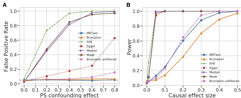
Figure 2. False-positive rate (FPR) and power comparison between various methods run on simulated data. (A) FPR (y-axis) under varying levels of confounding owing to population stratification (PS), with the x-axis describing the magnitude of the confounding effect of population labels on the exposure and outcome trait. (B) Power (y-axis) as a function of the magnitude of the causal effect of the exposure on the outcome trait (x-axis) in a setting with no confounding. Results are averaged over 1000 simulation replicates.
