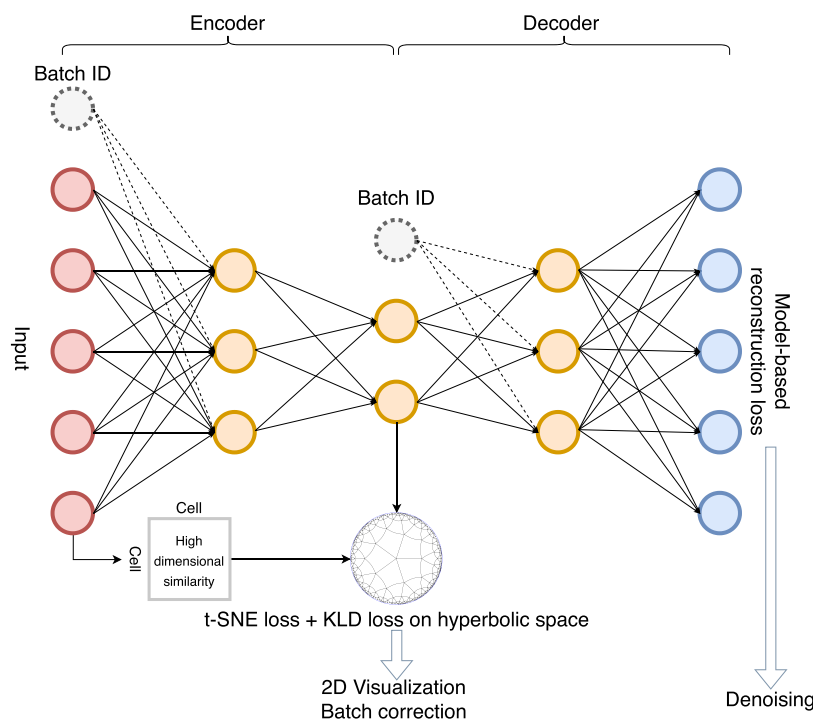
Figure 1. Network architecture of scDHMap. The encoder and decoder are fully connected neural networks. The latent embedding is in a 2D hyperbolic space for visualization and with the t-SNE regularization for structural preservations. KL divergence loss minimizes the divergence between the posterior and prior distributions of the latent embedding. Batch IDs can be incorporated to align different batches. Zero-inflated negative binomial (ZINB) reconstruction loss characterizes single-cell count data.
