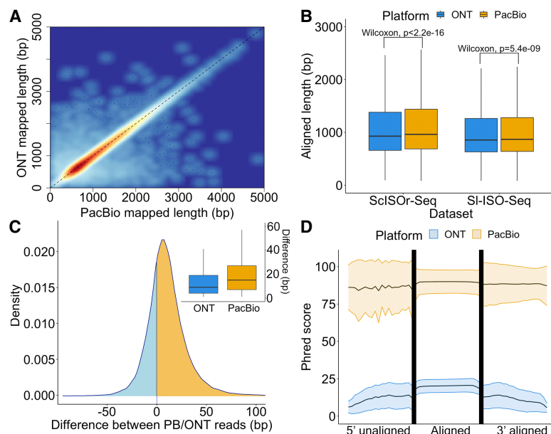
Figure 2. Alignment characteristics of RT read pairs. (A) Heatscatter plot showing aligned lengths of respective PacBio read ( x -axis) and ONT read ( y -axis) from the RT read pair after mapping to the genome using minimap2 (SI-ISO-Seq data set, Spearman's Rho: 0.96, p < 2.2 \times 10^{-16} ). (B) Comparison between aligned lengths of PacBio and ONT reads for both data sets after mapping to the genome using minimap2. (C) Density plot showing the difference between aligned lengths of PacBio read and ONT read from the RT read pair after mapping to the genome using minimap2 (SI-ISO-Seq data set) and box plot showing distribution of the differences. In the density plot, cases when PacBio alignment is longer correspond to the yellow area under the curve; the opposite is represented by the blue area. (D) Mean Phred score distribution along the read for aligned (middle) and unaligned (left and right) parts of PacBio (yellow) and ONT (blue) reads based on a (reference-free) pairwise Smith–Waterman alignment of the PacBio and ONT reads from the RT read pair (SI-ISO-Seq data set). Lower and upper bounds represent the standard deviation of the Phred score distribution.
