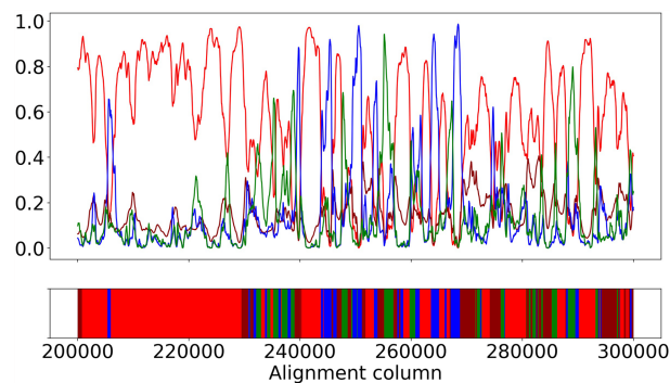
Figure 4. True genealogy and posterior distribution along the sequence. The upper panel shows posterior probability of each genealogy at each site. The lower panel shows the true genealogy of each site. Coloring corresponds to different genealogies: Genealogy HC1 is in red, HC2 is in dark red, HG is in blue, and CG is in green.
