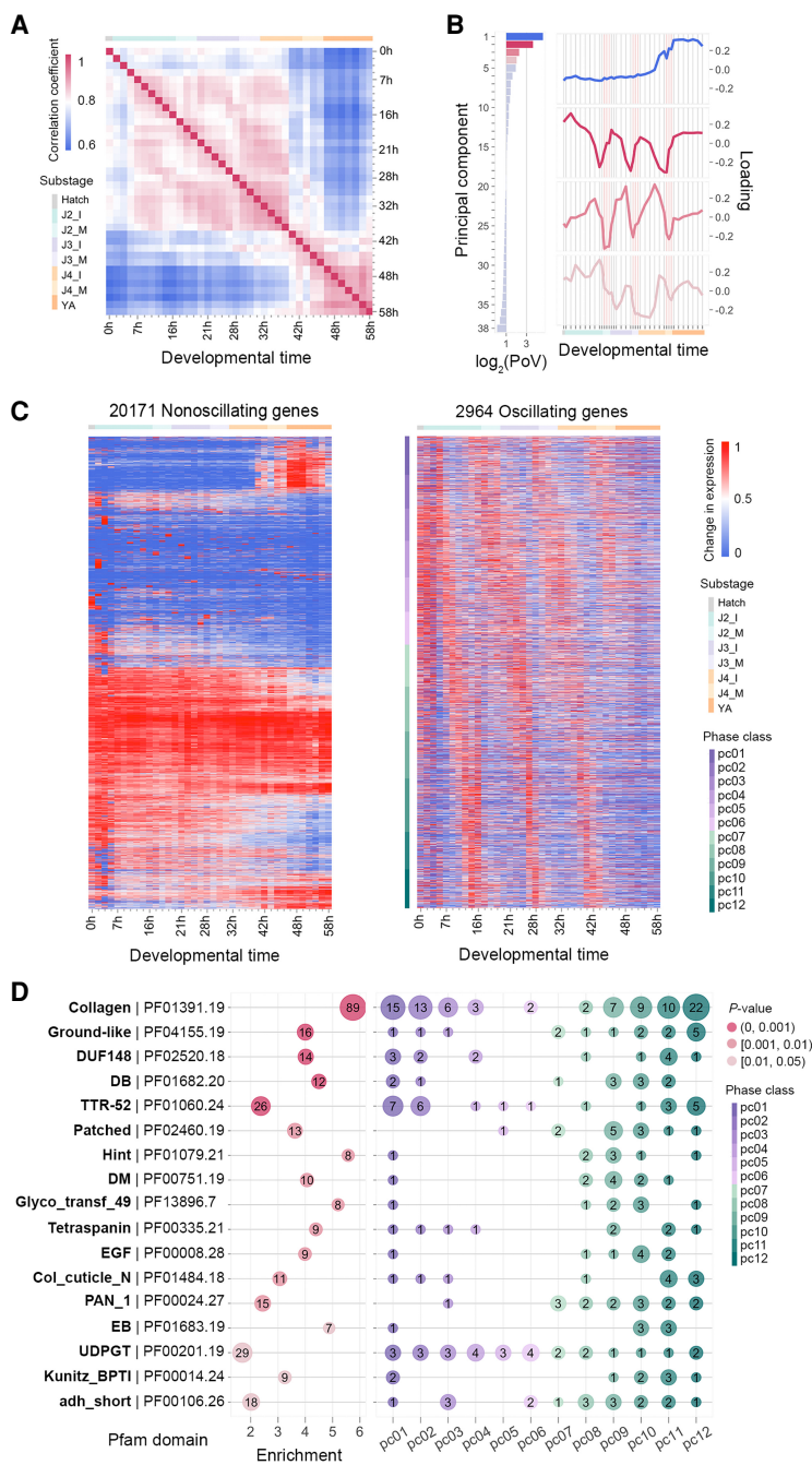
Figure 2. Thousands of oscillating genes are synchronized with the molting cycle in P. pacificus . (A) The heatmap displays the cross-correlation of log 2 -transformed expression patterns of all reliably expressed genes (reg; n = 23,135 ) obtained from the 38 time points. The time course was broken down into seven substages: J2 intermolt (J2_I), J2 molt (J2_M), J3 intermolt (J3_I), J3 molt (J3_M), J4 intermolt (J4_I), J4 molt (J4_M), and young adults (YA). (B) Proportion of variance (PoV) of gene expression by 38 principal components (PCs; left graph) and changes (loadings) of expression for each of the four top PCs (right graph). (C) The heatmaps visualize changes in gene expression throughout development for nonoscillating genes ( n = 20,171 ; left) and oscillating genes ( n = 2,964 ; right). The mean TPM was calculated from three biological replicates and was normalized by its maximum of each expression trace. The order of rows in the heatmap with the oscillating genes was sorted by phase class, which indicated a phase difference of 30, corresponding to a peak shift by \sim 1 h. (D) Oscillating genes were tested for overrepresentation of protein domains that are most significantly enriched among oscillating genes, the x-axis presents the enrichment score, and the y-axis shows the name of protein domains. The size of circles corresponds to the number of oscillatory genes with a given protein domain, and the three different colors indicate significance levels as measured by Fisher's exact test. The right graph profiles the overrepresented protein domains according to the 12 phase classes. The number of oscillatory genes in each phase class is marked.
