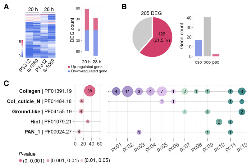
Figure 6. Integration of eud-1 as upstream regulator of oscillatory core genes. (A) The heatmap shows the expression levels of 205 differentially expressed genes (DEGs) between the eud-1 ( tu1069 )-mutant and wild-type (PS312) animals at 20 h and 28 h. The bar plot indicates the number of up-/down-regulated genes. (B) The pie chart displays the overlap between DEGs and oscillating genes. The bar plot shows the number of the oscillating DEGs among the three oscillating gene classes. (C) Protein domain enrichment analysis reveals that the collagen gene family is highly enriched in the 205 DEGs, the x-axis presents the enrichment score, and the y-axis shows the name of protein domains. The size of the circles corresponds to the number of oscillatory genes in a given protein domain, and the three different colors indicate different significance levels as measured by the Fisher's exact test. The right graph profiles the overrepresented protein domains according to the 12 phase classes. The number of oscillatory genes in each phase class is marked.
