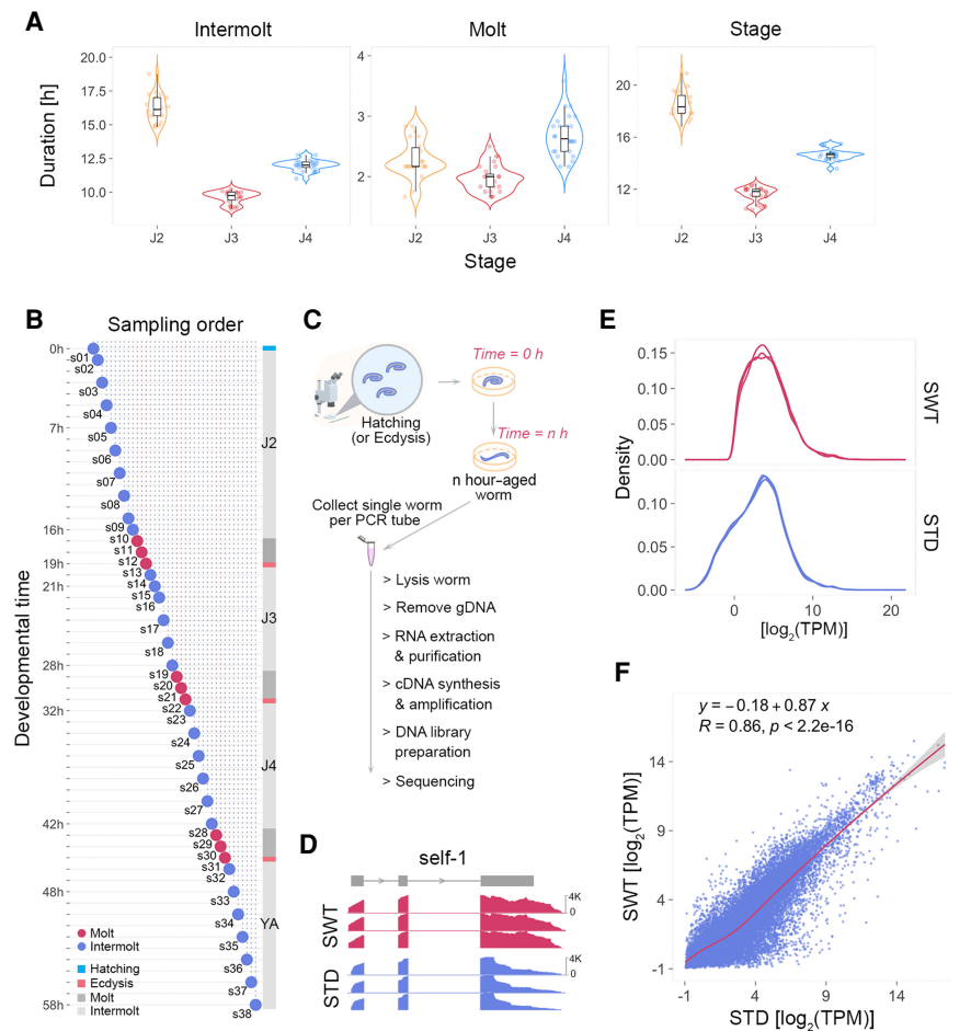
Figure 1. Single worm transcriptomic (SWT) sequencing in P. pacificus . (A) The violin plots display the duration of intermolt, molt, and the whole stage for all three juvenile stages (J2, J3, and J4). The head structure of the wild type at hatching, lethargus, and ecdysis is shown in Supplemental Figure S1. (B) The schematic shows the distribution of time points for SWT samples, which cover 58 h of postembryonic development from hatching to young adults. The three time points of each molt indicated in red represent the substages of molting: lethargus, apolysis, and ecdysis, respectively (for visualization, see Supplemental Fig. S1). Animals were collected hourly or every 2 h in the molt or intermolt stage. (C) Schematic summary of the workflow for SWT. (D) RNA-seq read coverage is visualized at the self-1 locus using the Integrative Genomics Viewer (IGV) (Robinson et al. 2011) as one example for comparing SWT and standard RNA-seq (STD). (E) Density of gene expression of SWT and STD samples, six replicates each. (F) The scatterplot shows the correlation of the mean TPM of individual genes between SWT and STD data at the lethargus of the fourth molt. Three biological replicates for each method.
