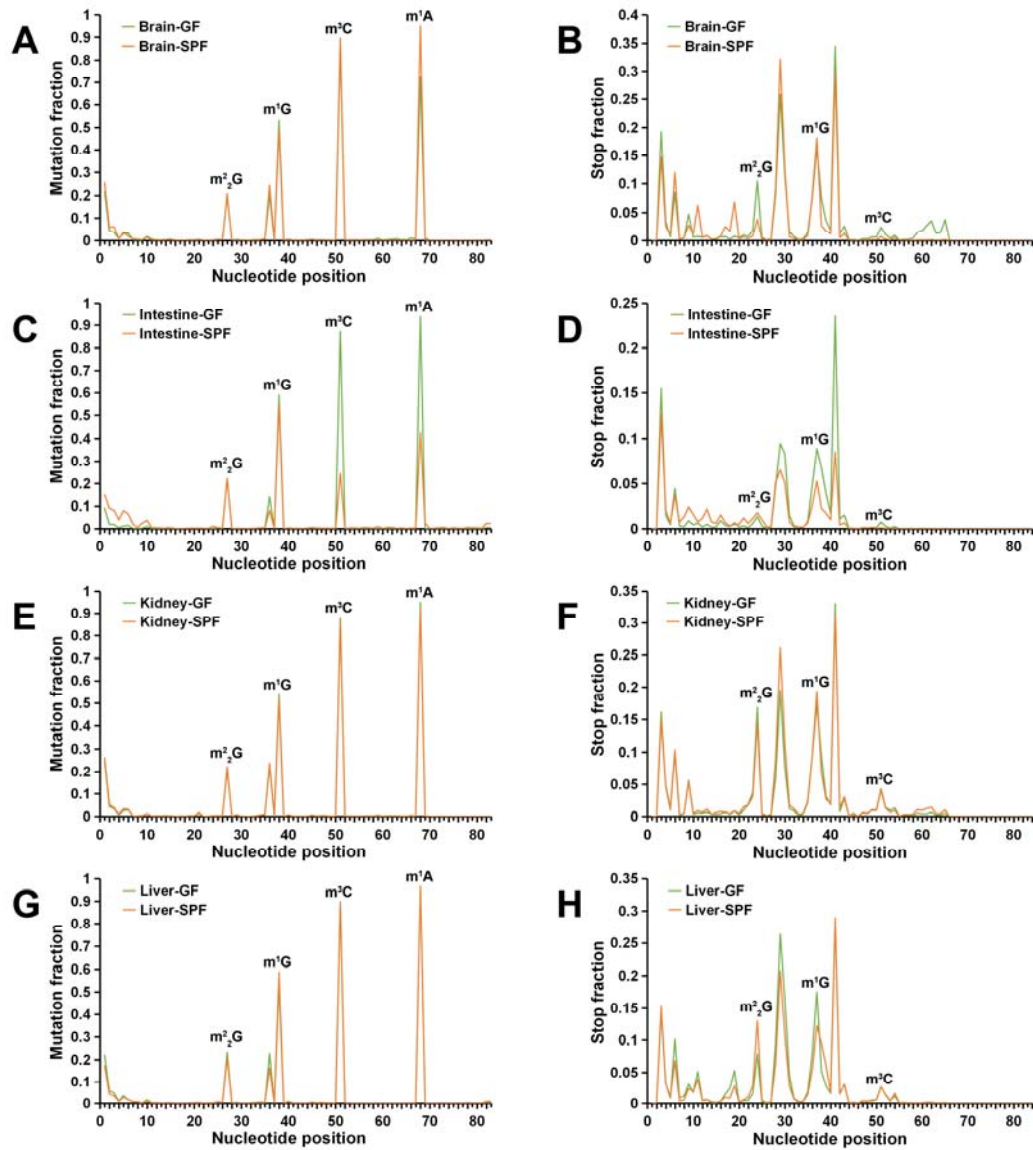
Figure 6. Mutation and stop plots for the cytosolic tRNA Leu-CAG isoacceptor in four tissues ( n = 3 for both GF and SPF mice) from the -DM libraries. (A) Mutation plot for the brains. (B) Stop plot for the brains. (C) Mutation plot for the intestines. (D) Stop plot for the intestines. (E) Mutation plot for the kidneys. (F) Stop plot for the kidneys. (G) Mutation plot for the livers. (H) Stop plot for the livers. The stop fractions at and after m 1 A58 are not shown. The x -axis corresponds to the nucleotide position along the tRNA. Watson-Crick face methylations that are sensitive to demethylase treatment can be easily identified from the mutation plots. m 2 2 G: N 2 ,N 2 -dimethylguanosine.
