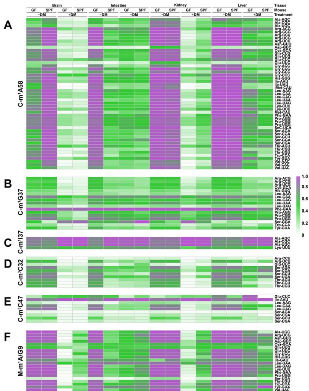
Figure 5. Mutation heatmaps of common methylation types within cytosolic or mitochondrial tRNAs according to the standard tRNA nomenclature. The modification-level of each type of tRNA methylation was semi-quantified based on the corresponding mutation fraction, and presented data are from four tissues ( n = 3 for both GF and SPF mice). (A) N^1 -methyladenosine of position 58 ( m^1A58 ) within cytosolic tRNAs. (B) N^1 -methylguanosine of position 37 ( m^1G37 ) within cytosolic tRNAs. (C) N^1 -inosine of position 37 ( m^1I37 ) within cytosolic tRNAs. (D) N^3 -methylcytosine of position 32 ( m^3C32 ) within cytosolic tRNAs. (E) N^3 -methylcytosine of
