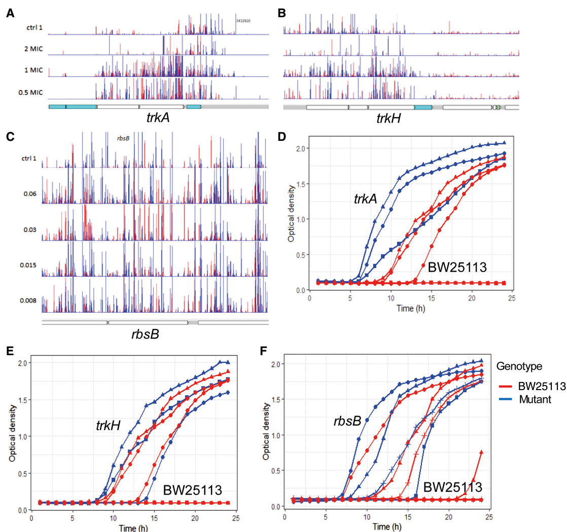
Figure 3. Novel importers contributing to triclosan sensitivity. (A,B) Insert patterns indicating inactivation of trkAH is beneficial for survival in the presence of triclosan. (C) Increase in insertions within the first part of rbsB in triclosan-exposed libraries. (D–F) Growth curves for BW25113 and isogenic mutants grown in LB broth supplemented with 0.125 mg/L of triclosan. Mutants were replicated on multiple plates. Each line indicates the average from an individual plate; independent plates are represented by symbols (triangles, circles, or squares; allowing comparison between the mutant and parent from each individual plate). Red lines indicate BW25113; blue lines, mutants. The format of the genetic maps is as described in Figure 1.
