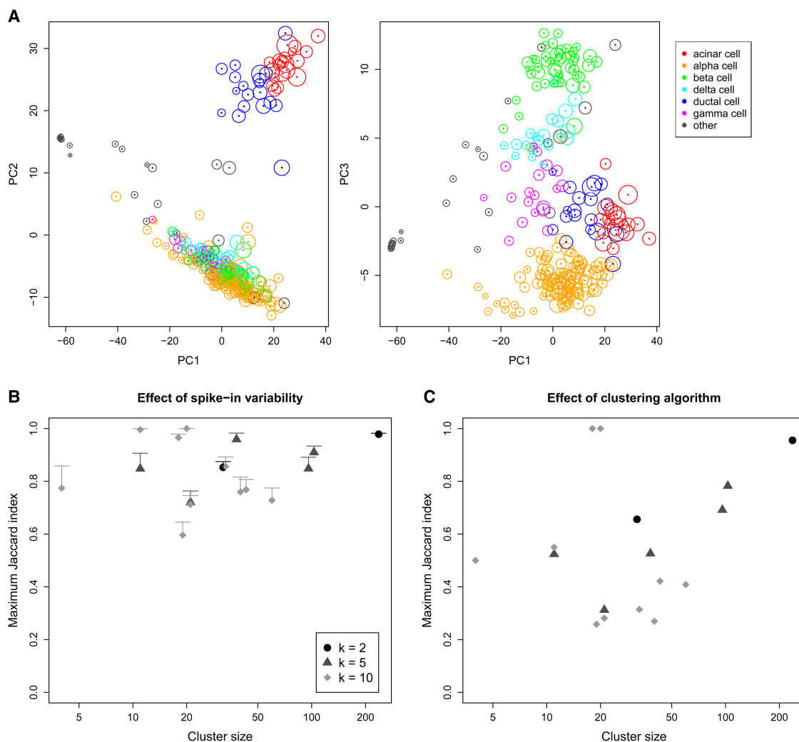
Figure 4. Effect of spike-in variability on dimensionality reduction and clustering in simulated data, based on real scRNA-seq data for cells extracted from a healthy human pancreas (Segerstolpe et al. 2016). (A) PCA plots of the first three principal components, in which each cell is colored according to its annotated cell type from the original study. The circle around each cell contains 95% of remapped locations across the simulation iterations, and represents the deviation in location due to spike-in variability. (B) Clusters were identified from the original data by hierarchical clustering with Ward's criterion, followed by a tree cut with k of 2, 5, or 10. This was repeated at each simulation iteration, and the maximum Jaccard index between each original cluster and any of the simulated clusters at the same k was computed. Each value represents the mean of 20 simulation iterations, and the error bars represent standard errors. (C) The maximum Jaccard index for each original cluster generated with Ward's criterion compared to clusters generated from complete-linkage clustering of the original data.
