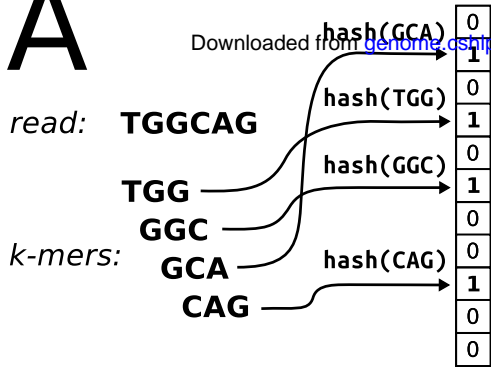
Bloom filter
