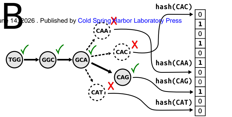
Bloom filter
