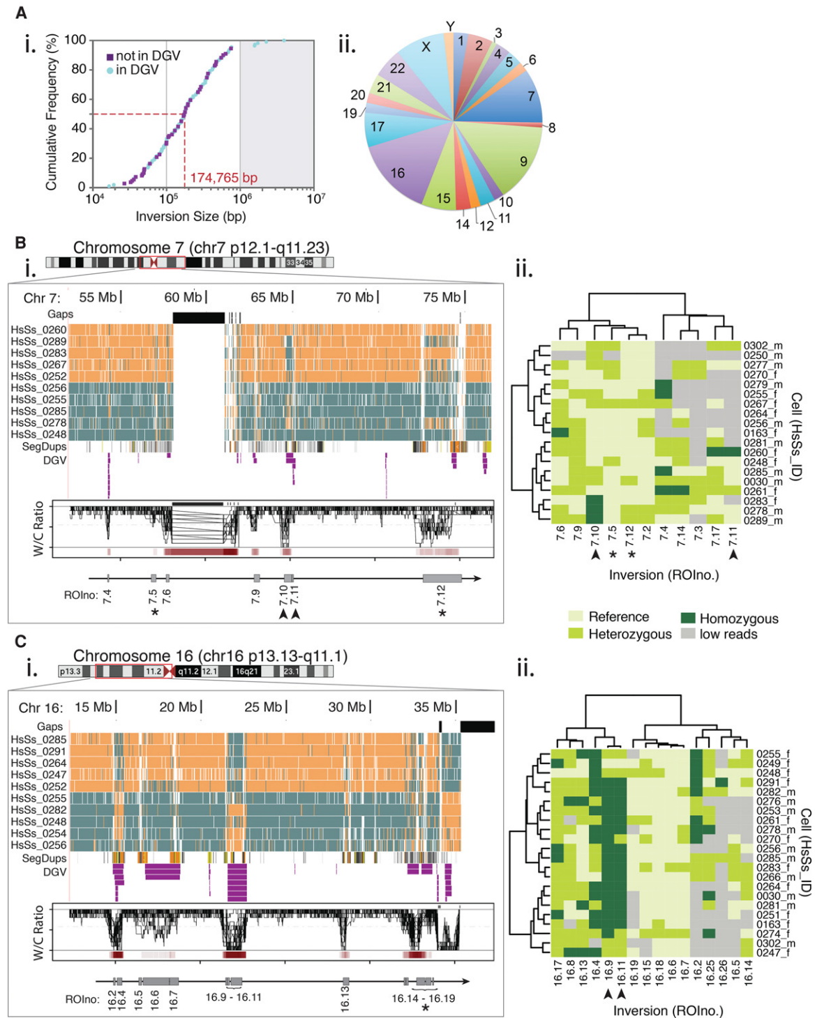
Figure 3. Polymorphic inversions mapped in multiple single cells of a pooled donor population. (A) Size and genomic distributions of 111 polymorphic inversions identified in the pooled donor population. (i) The cumulative frequency of inversion sizes in base pairs (bp), divided into new inversions (purple squares) and those overlapping with the Database of Genomic Variants entries (blue circles). The median inversion size (dashed red line) is well below the 1-Mb detection limit of traditional cytogenetic techniques (gray shading). (ii) Distribution of the total number of inversions present on each chromosome. (B, C) Polymorphic domains (red box) mapped to Chr 7 (B) and Chr 16 (C). Asterisks and arrowheads denote specific inversions highlighted in the main text. (i) Detail of the domains shown in the UCSC Genome browser ‘packed’ view for 10 representative Strand-seq libraries, along with tracks for sequence gaps (black), segmental duplications (SegDups), and inversions identified in the DGV (purple). Corresponding overlaid Invert.R histograms of W/C ratios and inversion frequency heat maps (red bars) are shown in the lower panel. The polymorphic inversions (gray boxes) and corresponding ROIno identifiers are shown below. (ii) Clustered heat maps of the genotyped inversions (x-axis) identified in each cell (y-axis). Inversions are depicted as pale green (homozygous reference), medium green (heterozygous), or dark green (homozygous). In some cases, too few reads were present in the region to genotype the ROI (gray).
