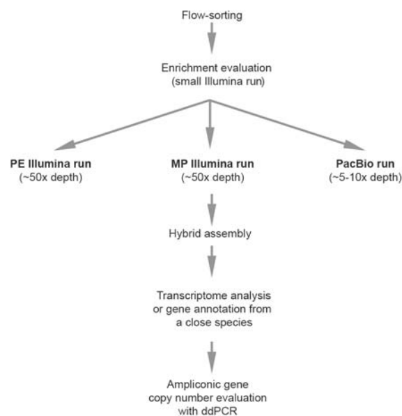
Figure 5. The workflow for sequencing mammalian Y Chromosomes.
