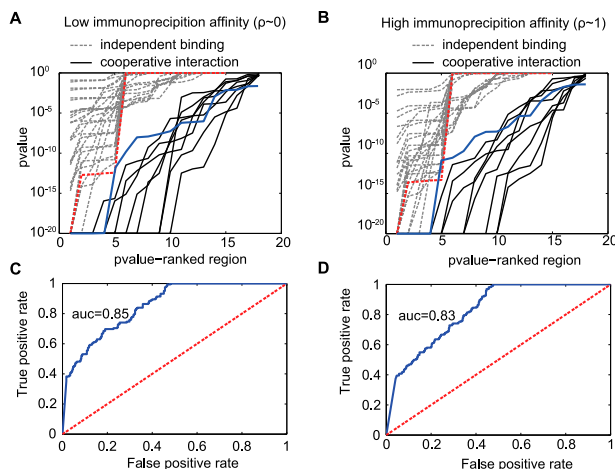
Figure 5. The double-binding signal allows the detection of cooperative interaction from the ChIP-seq data. Our method (Equation 8) is able to distinguish regions containing cooperative interacting sites from regions containing independent binding sites. A set of regions with experimentally validated cooperative interaction is used as a positive control (Chauhan et al. 2011). The negative control is obtained from simulation (Supplemental Figs. S3, S4; Supplemental Table S2; also see Methods). (A,B) The P -value output of our method is able to discriminate regions with cooperative interaction (solid lines) from regions with independent binding (dashed lines). Each dashed line represents a different simulated set. Each solid line assumes a different value for the probability of nonbinding configuration (see Methods). The probability of nonbinding configuration is a necessary input to compute the statistical P -value. Independent of the value for nonbinding configuration, our method discriminates the data well. A good discriminative power occurs even for the most conservative case (highlighted by the dashed red and solid blue lines). (C,D) The overall performance of our method is measured in terms of true versus false positive rate. The solid blue line represents the results from A or B. The dashed red line shows what is expected by chance. The area under the curve (AUC) measures the discriminative power of the method. All results support our method. In addition, the method is robust when performance evaluation is specific to each probability of nonbinding configuration (Supplemental Figs. S5, S6). The results at the left (A,C) and right (B,D) panels are obtained assuming low or high immunoprecipitation rate, respectively.
