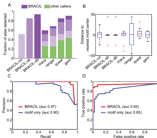
Figure 3. BRACIL increases the resolution of binding-site detection as well as sensitivity and specificity. The performance achieved by using only ChIP-seq coverage (BRACIL-co) is improved by including motif integration with the single-binding signal (BRACIL-sb), and the best performance occurs when we also consider the double-binding signal (BRACIL-db). A summary of the differences between the three versions can be found in Table 1. In the best scenario, BRACIL detects 44/47 of the reference sites (Chauhan et al. 2011). The potential of our method to refine the output of peak callers can be seen both in terms of the fraction of sites detected (A) as well as the resolution with which they are detected (B). The green bars (A) represent the fraction of sites detected by the corresponding peak caller labeled at the x-axis. The purple bars on the top show the additional refinement provided by our method. The different shades in purple represent performance improvement by specific variations of BRACIL. Enriched regions are defined as the overlapping window of \pm 150 bp around the single nucleotide prediction obtained by the corresponding peak caller. For BRACIL-co, BRACIL-sb, and BRACIL-db, the enriched regions consist in the \pm 150 -bp overlapping window that surrounds the reference sites. The precision and recall (C) and the ROC (D) plots illustrate that our method is especially important for filtering out low conservation motifs that do not represent real binding.
