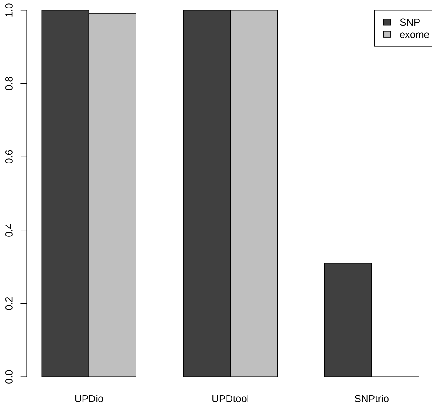
Specificity Comparison of Methods Tested at Default Settings
