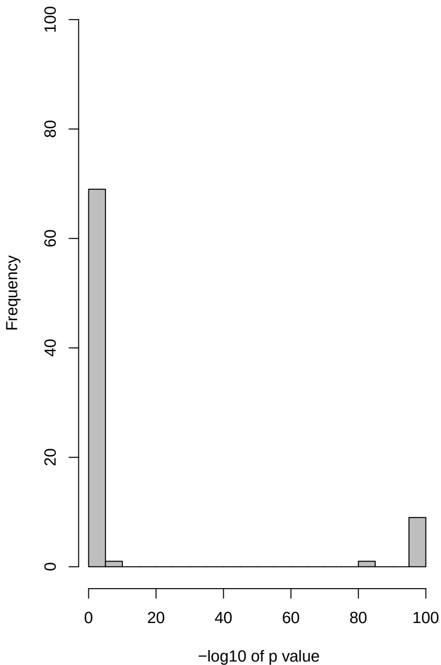
p value distribution from exome samples
