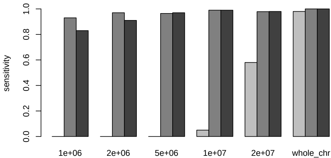
Heterodisomy from SNP
