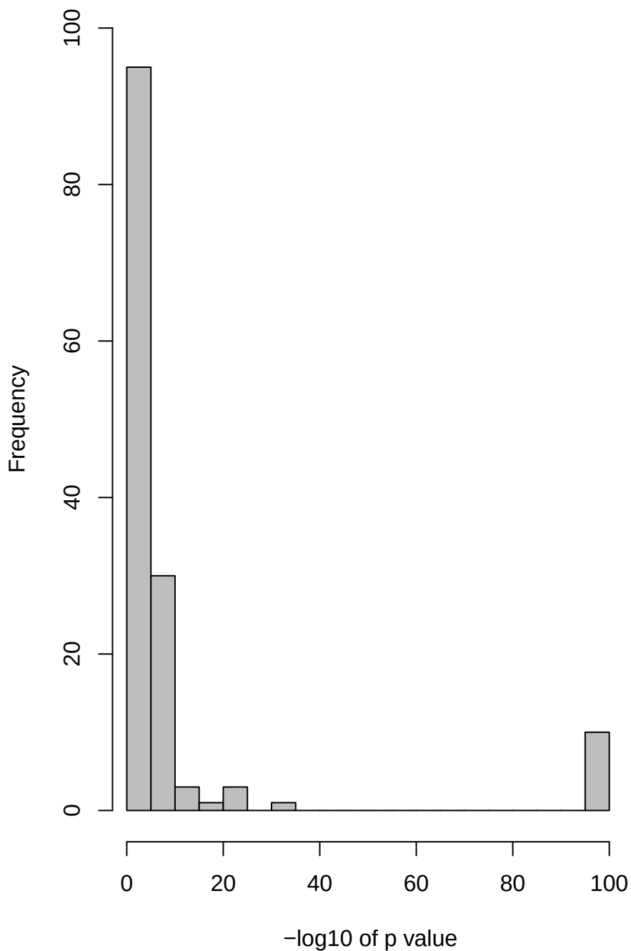
p value distribution from SNP samples
