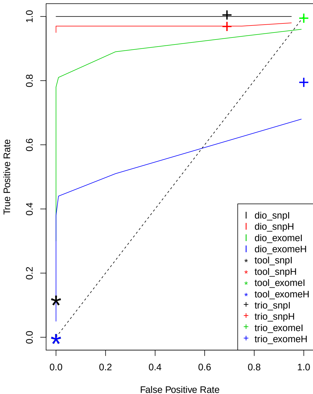
Simulated UPD Events at 5 Mb
