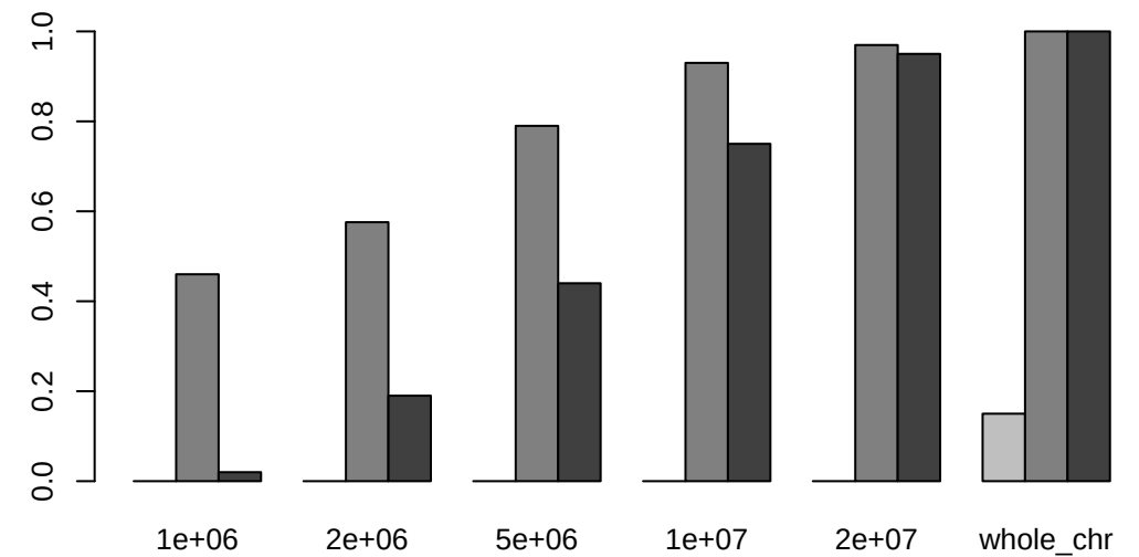
Heterodisomy from exome
