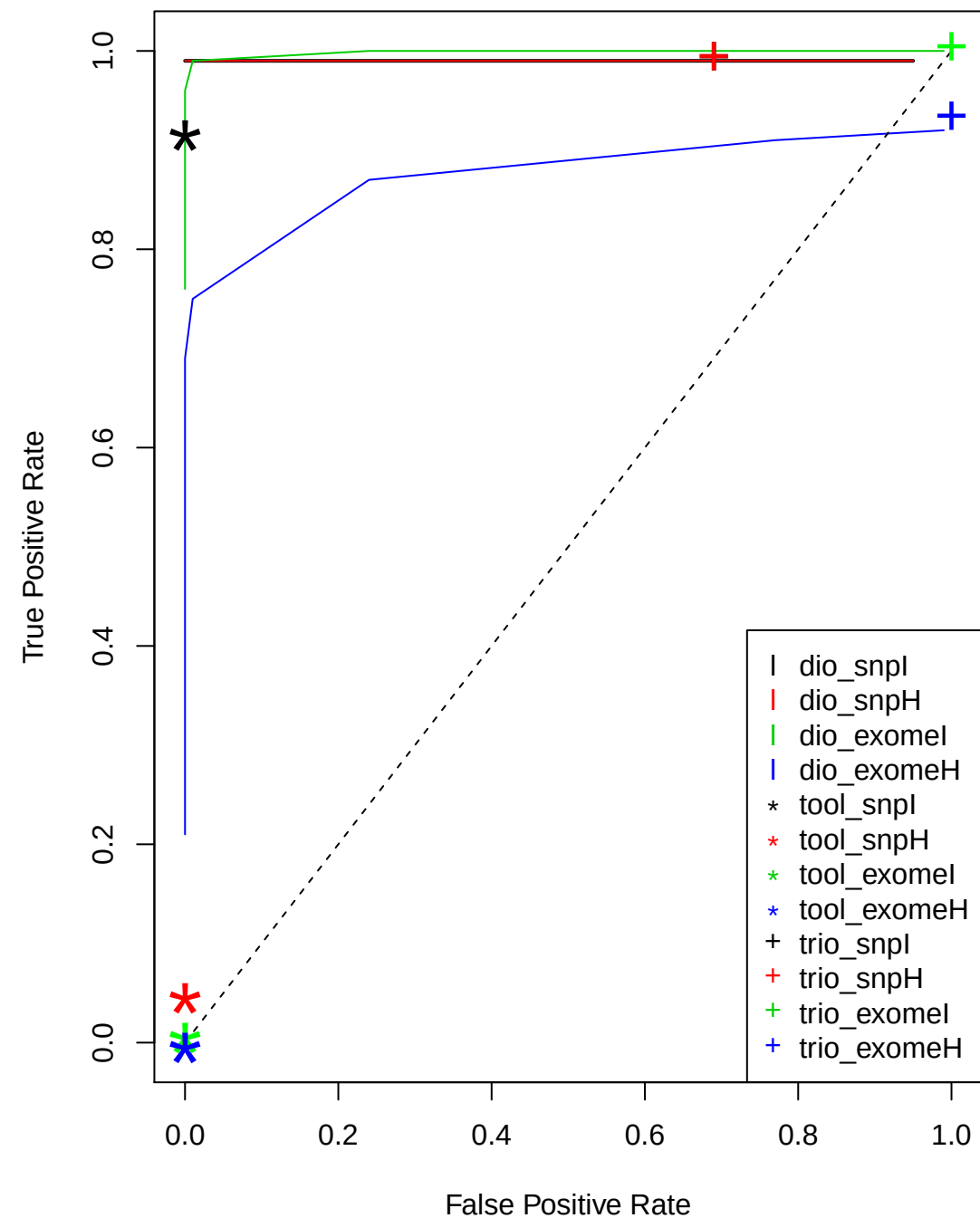
Simulated UPD Events at 10 Mb
