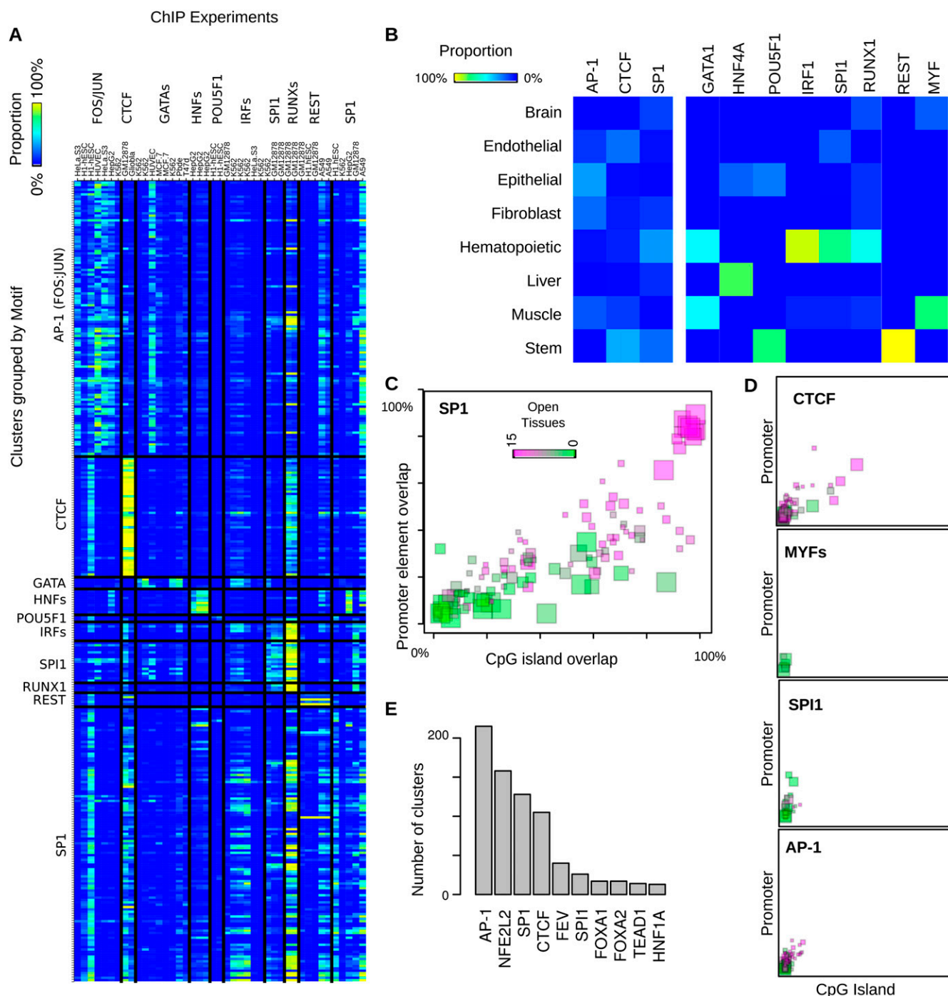
Figure 6. Motif specificity in SOM clusters. (A) Concordance ([yellow] high, [blue] low) between ChIP results (x-axis) and motif discovery in DNase I clusters (y-axis). (B) The cell-type specificity for selected motifs. This heatmap shows the distribution of most-open tissues for each motif. For example, 100% of the clusters where the POU5F1 motif was found had stem cells (Stem) as the most open tissue type, whereas MYF family motifs were found predominantly in muscle clusters. (C,D) Each colored square represents a cluster with enrichment for the given motif. (x-axis) overlap with CpG islands; (y-axis) overlap with promoters; (color) the number of tissues with at least one sample above a cutoff. Each factor shown here has a different distribution of cell-type specificity and promoter/CpG-island overlap. The size of a square indicates the number of DHSs in the cluster. (E) Number of clusters that are enriched for the most common motifs.
