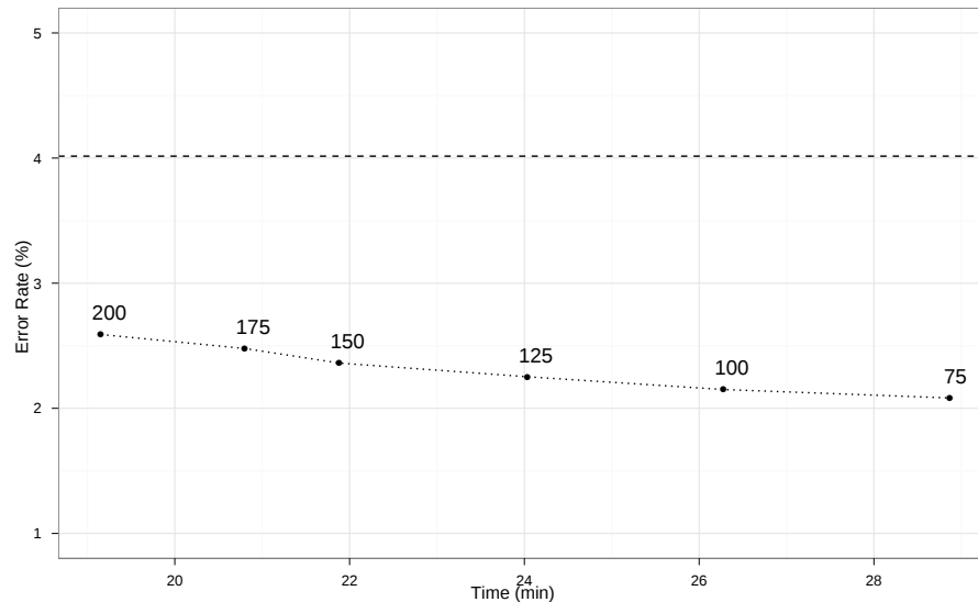
Figure 2: Accuracy versus time tradeoff for the Nesterov Algorithm on chromosome 4 from the Chinese Han group in HapMap3. The numbers indicate the sub-window size w . The dashed line marks the error rate for MaCH on the same data set.
