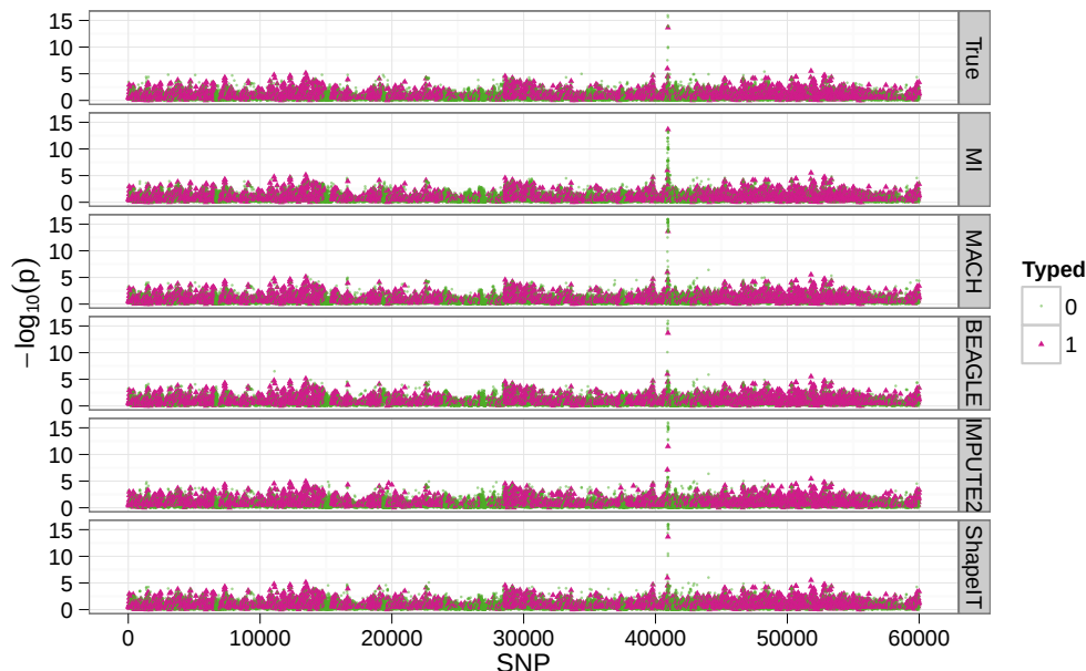
Figure 1: The negative logarithm of p-values for association when the true signal depends on SNP 40938. MENDEL-IMPUTE is abbreviated MI.
