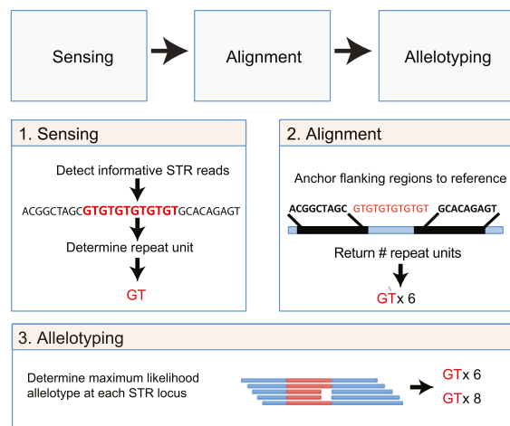
Figure 1. lobSTR algorithm overview. lobSTR consists of three steps. The sensing step detects informative STR reads and determines their repeat motif. The alignment step maps the STRs' flanking regions to the reference. The allelotyping step determines the STR alleles present at each locus.
