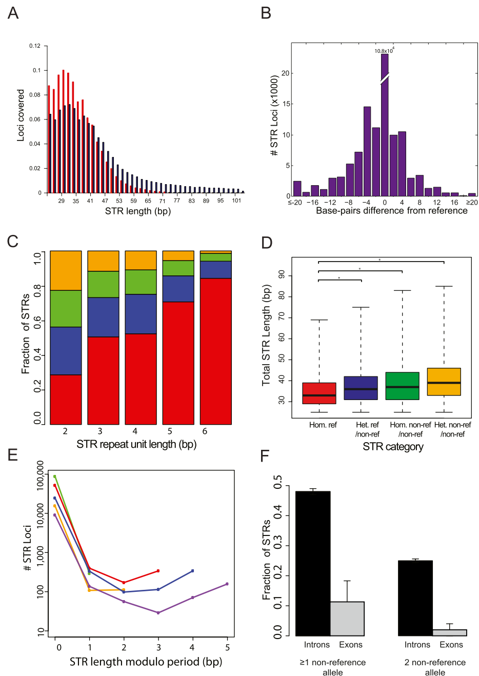
Figure 5. Genome-wide STR profile of an individual. (A) Distribution of STRs with 20 \times coverage or more as a function of the allele size in hg18. (B) Distribution of allele size differences from reference in lobSTR calls. The average difference was 6.3 bp away from the reference. (C) STR polymorphism as a function of period. The number of STR alleles matching the reference sequence increases with increasing repeat unit length. (Red) Homozygous reference; (blue) heterozygous nonreference/reference; (green) homozygous nonreference/nonreference; (orange) heterozygous nonreference/nonreference. (D) Longer STR regions are more polymorphic. The median STR length (thick black line) increases with the number of variant alleles. (*) A significant ( p < 0.05 ) difference according to a one-sided Mann–Whitney test. Boxes denote the interquartile range, and whiskers denote three times the interquartile range. (E) lobSTR shows mutational trends at single-base-pair resolution. The number of base pairs different from the reference modulo period size versus the number of alleles detected (in logarithmic scale) is shown for each period; (green) period 2; (orange) period 3; (red) period 4; (blue) period 5; (purple) period 6. Incomplete STR unit differences tend to differ by a full unit \pm 1 bp from the reference. (F) Fraction of trinucleotide STRs with nonreference alleles in introns versus exons. The 95% confidence intervals are given by the error bars.
