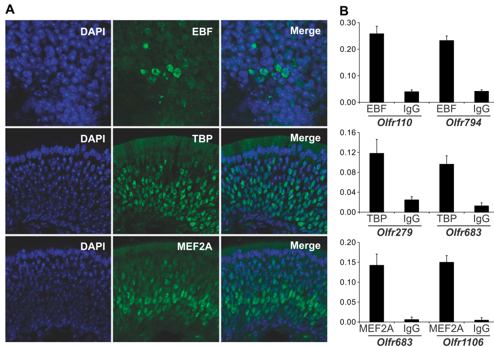
Figure 4. EBF, TBP, and MEF2A proteins are expressed in the MOE and physically associate with the promoters of Olf110 , Olf279 , Olf683 , Olf794 , or Olf1106 in vivo. (A) Immunohistochemistry of MOE from mice at postnatal day 21, with anti-EBF, anti-TBP, and anti-MEF2A antibodies (green). Nuclei were visualized with DAPI (blue). Scale bars, 30 \mu\text{m} (top row), 60 \mu\text{m} (center and bottom row). (B) ChIP assays were performed on MOE from mice at 22–30 d postnatally. Chromatin was immunoprecipitated with anti-EBF, anti-TBP, and anti-MEF2A antibodies. Normal rabbit IgGs were used as negative control. Enrichment of promoter sequences in the immunoprecipitates was determined by qPCR, using specific primers. The relative abundance of target DNA was expressed as percentage of total input chromatin. Data were obtained from two independent experiments. Statistical analysis: p < 0.05 in all cases.
