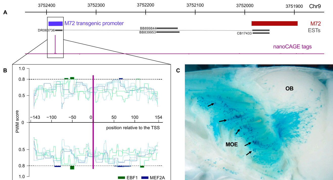
Figure 5. Transgenic reporter assay of the promoter activity of sequences flanking a nanoCAGE TSS. (A) Schematic depiction of the locus of Olfr160 ( M72 ) on mouse chromosome 9. (Red) OLFR160 coding sequence; (blue) Olfr160 transgenic promoter; (purple) nanoCAGE tags; (black) ESTs. (B) Position weight matrix (PWM) scanning of the promoter sequences with matrices for EBF1 (green) and MEF2A (blue). Highlighted are the regions where the signal is above a 0.8 score threshold. (C) Whole mount of a mouse from transgenic line 7 shows X-gal-labeled cells predominantly in the middle domain of the MOE (black arrows). Labeled axons spread over a large domain in the middle aspect of the medial half-olfactory bulb, a probable consequence of the absence of an intact OR CDS in the transgene. The dotted gray line follows the shape of the cribriform plate separating the MOE from the olfactory bulb (OB).
