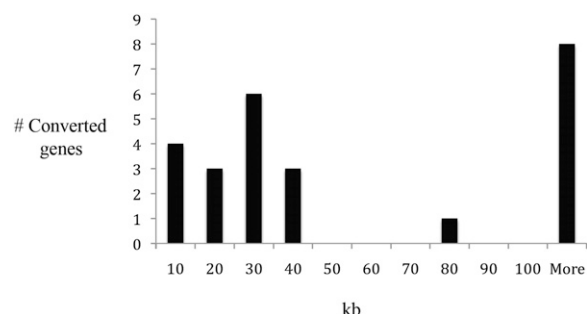
Figure 3. Distance in kilobases (kb) between donor and acceptor sequences for the 25 intrachromosomal IGC pairs with assigned donor sequences.
