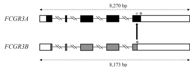
Figure 4. Interlocus gene conversion from FCGR3B to FCGR3A . The FCGR3A gene encodes a receptor for the Fc portion of immunoglobulin G, which is involved in the removal of antigen–antibody complexes from the circulation. The highly similar paralog, FCGR3B , which resides only 73 kb downstream from FCGR3A , encodes a shorter protein due to differences in the positions of both the start and stop codons. Coding exons are shown as filled boxes, UTRs as empty boxes. Introns are represented as lines and are not drawn to scale. The black asterisks indicate the normal stop codons of the FCGR3A and FCGR3B genes; the gray asterisk identifies the premature stop codon in the FCGR3A gene that is introduced by an IGC event with FCGR3B .
