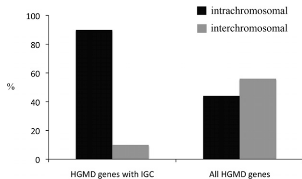
Figure 2. Excess of interlocus gene conversion (IGC) between intra-chromosomal paralogous sequences. HGMD genes with IGC: 30 genes with deleterious mutations introduced by IGC. All HGMD genes: 3196 genes from the HGMD database.
