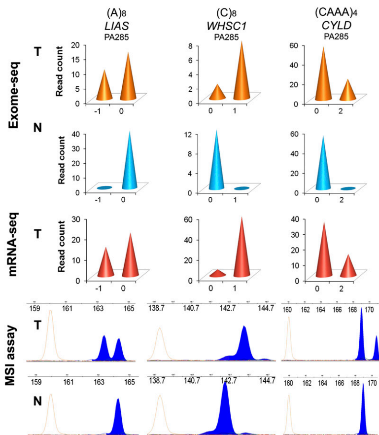
Figure 4. MSI analysis using Exome-seq. The data for three representative microsatellites are shown. ( Top ) Read-depth based Exome-seq data; ( middle ) mRNA-seq data; ( bottom ) electropherograms of the conventional MSI assay. For the top and middle panels, the x -axis indicates the lengths of indels. The negative value indicates base deletion, and the positive value indicates base insertion, while 0 indicates no indel. The numbers marked at the y -axis indicate the number of sequence reads that carry the mutant allele or the wild-type allele. ( Bottom ) x -axis is the size in bases; y -axis is the fluorescence intensity. The red peaks are internal size standards.
